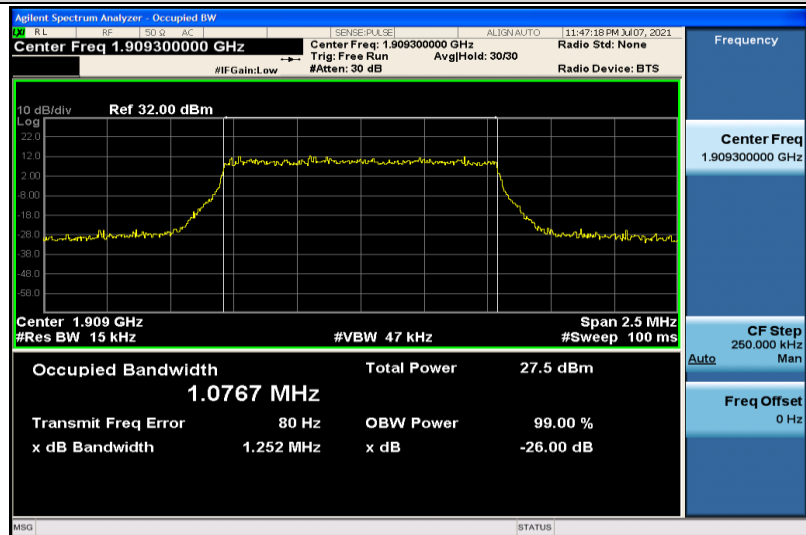
Band2-1.4MHz-16QAM-19193-6RB#0-1.0767
