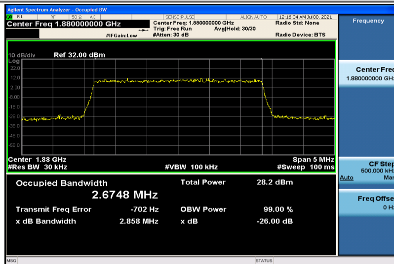
Band2-3MHz-16QAM-18900-15RB#0-2.6748
