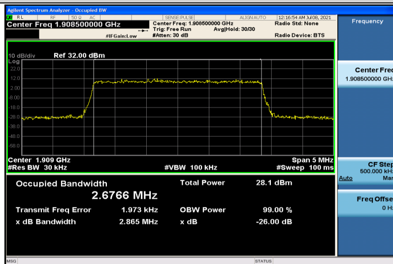
Band2-3MHz-16QAM-19185-15RB#0-2.6766
