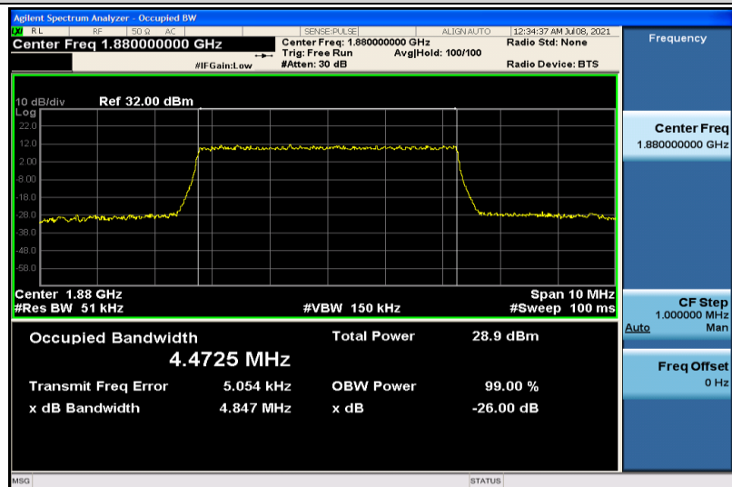
Band2-5MHz-16QAM-18900-25RB#0-4.4725
