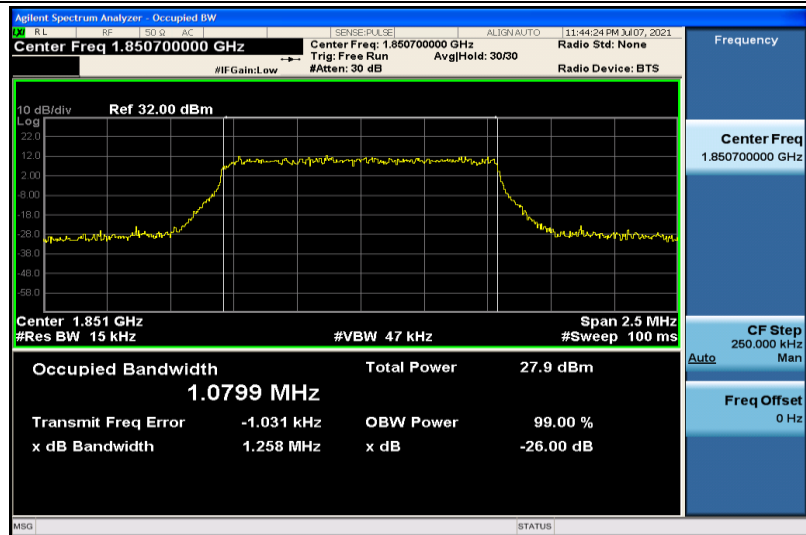
Band2-1.4MHz-16QAM-18607-6RB#0-1.0799
