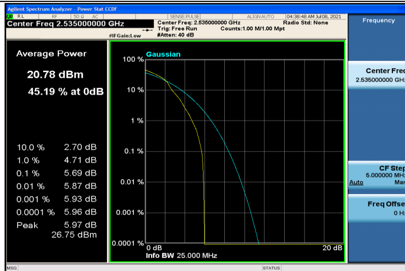
Band7-5MHz-16QAM-21100-1RB#0
