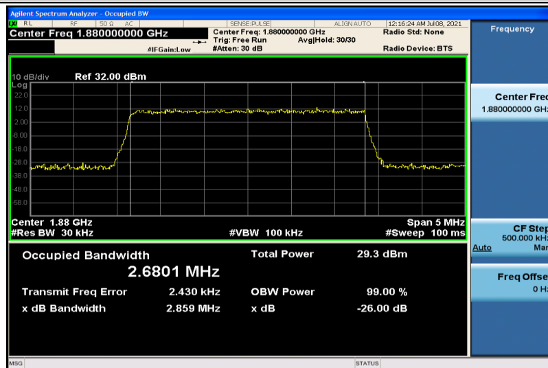
Band2-3MHz-QPSK-18900-15RB#0-2.6801
