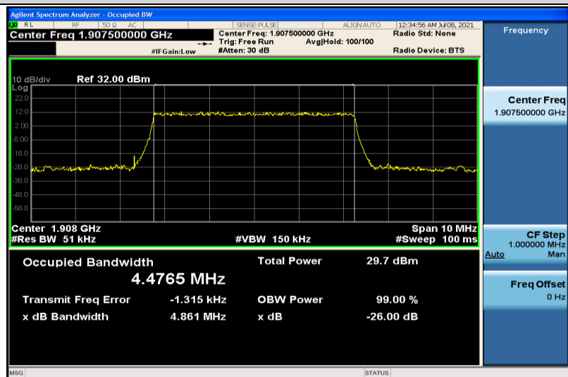
Band2-5MHz-QPSK-19175-25RB#0-4.4765
