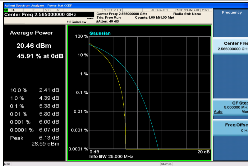
Band7-10MHz-QPSK-21400-50RB#0
