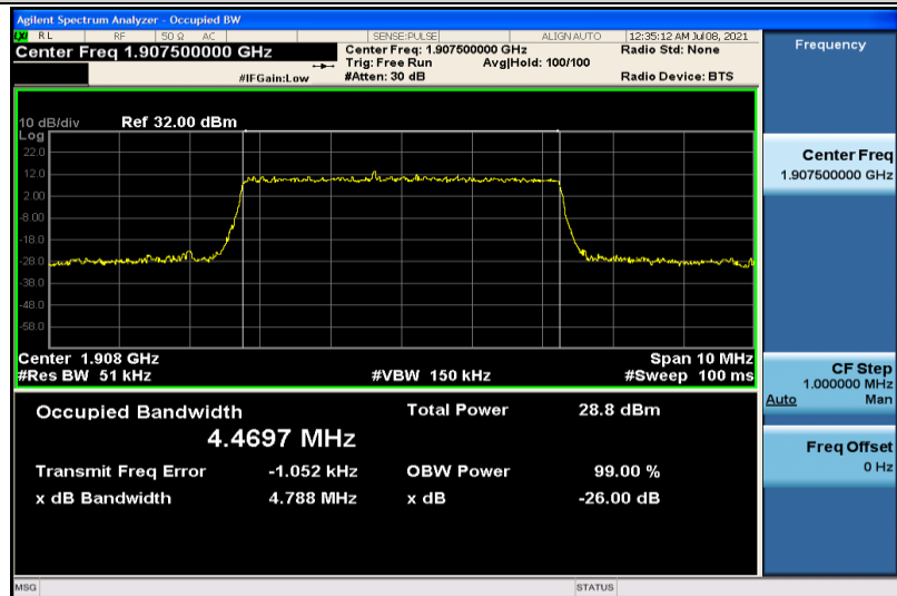
Band2-5MHz-16QAM-19175-25RB#0-4.4697
