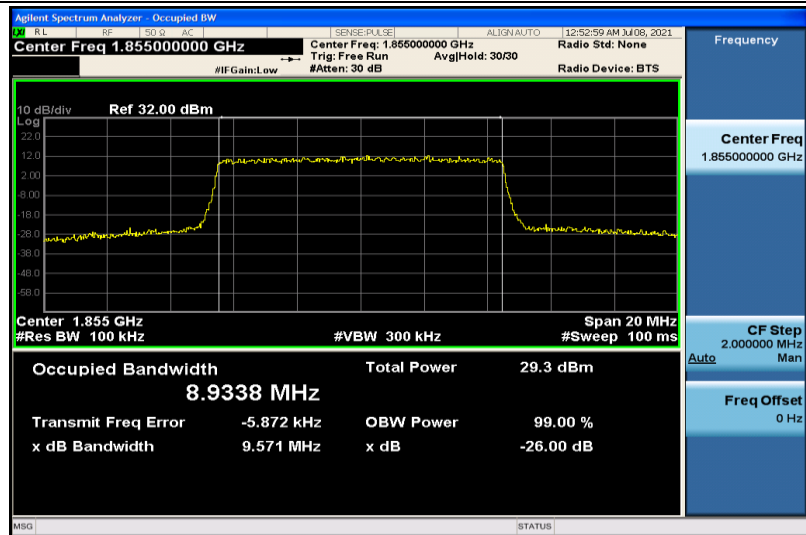
Band2-10MHz-16QAM-18650-50RB#0-8.9338
