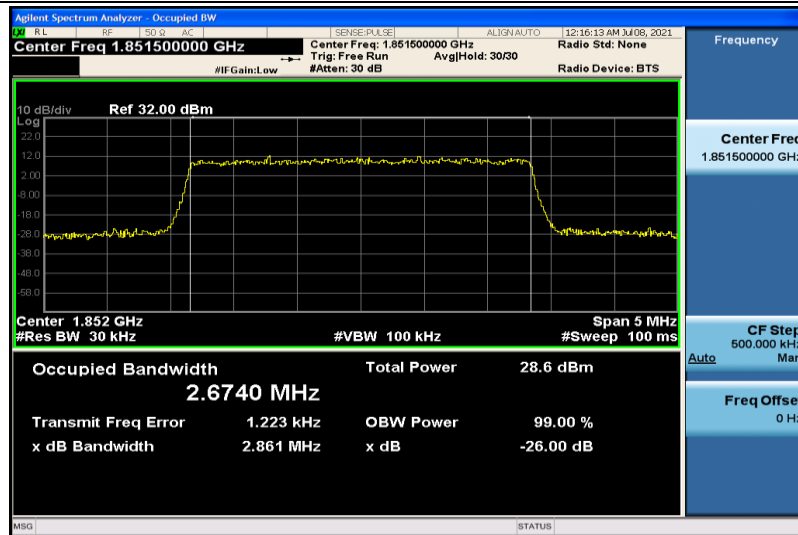
Band2-3MHz-16QAM-18615-15RB#0-2.6740
