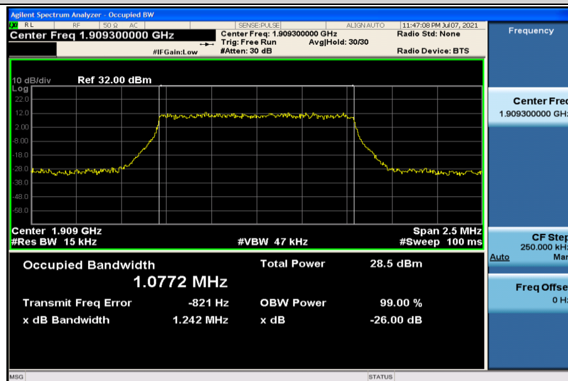
Band2-1.4MHz-QPSK-19193-6RB#0-1.0772
