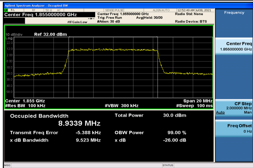
Band2-10MHz-QPSK-18650-50RB#0-8.9339
