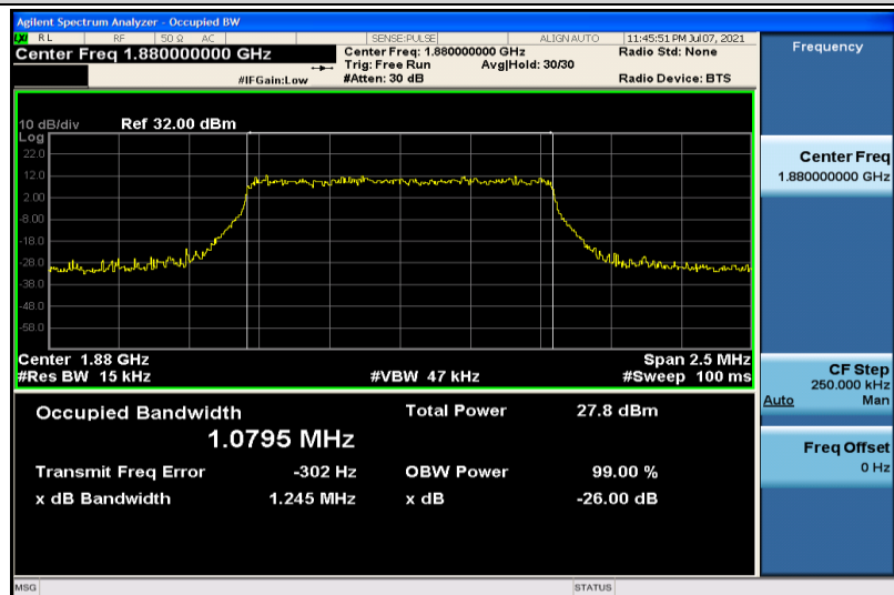
Band2-1.4MHz-16QAM-18900-6RB#0-1.0795
