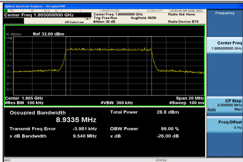
Band2-10MHz-16QAM-19150-50RB#0-8.9335
