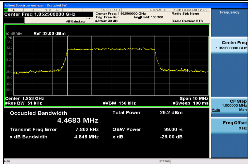
Band2-5MHz-16QAM-18625-25RB#0-4.4683
