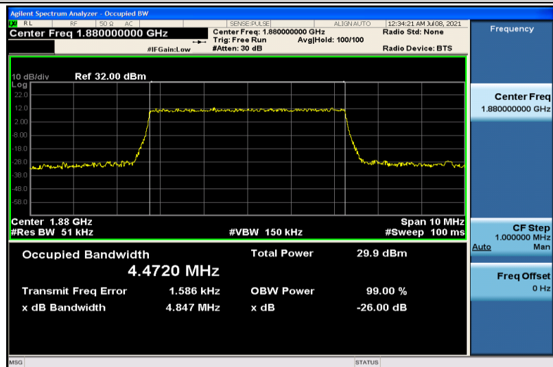
Band2-5MHz-QPSK-18900-25RB#0-4.4720
