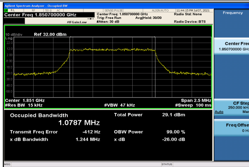
Band2-1.4MHz-QPSK-18607-6RB#0-1.0787
