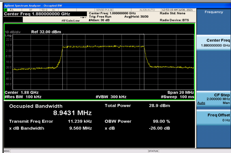
Band2-10MHz-16QAM-18900-50RB#0-8.9431
