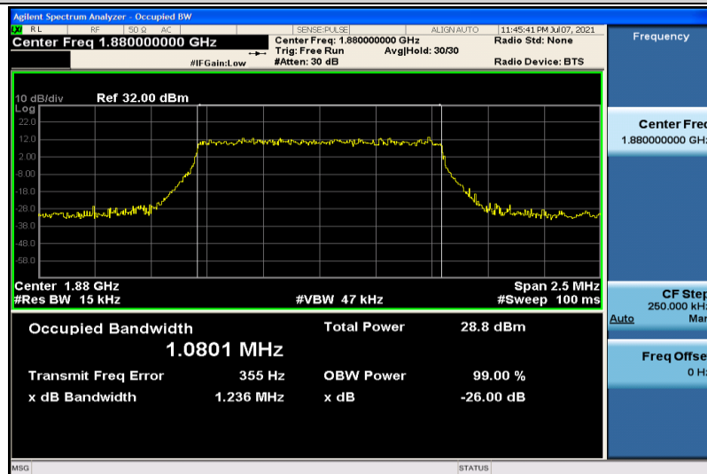
Band2-1.4MHz-QPSK-18900-6RB#0-1.0801
