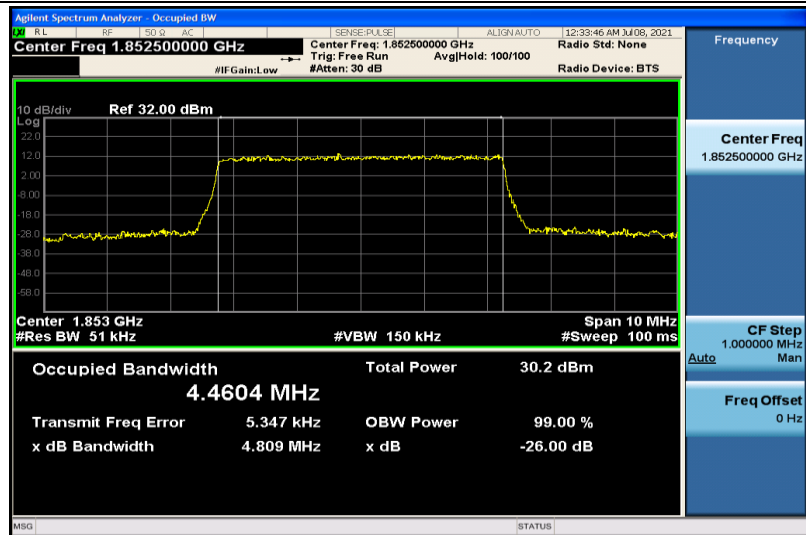
Band2-5MHz-QPSK-18625-25RB#0-4.4604
