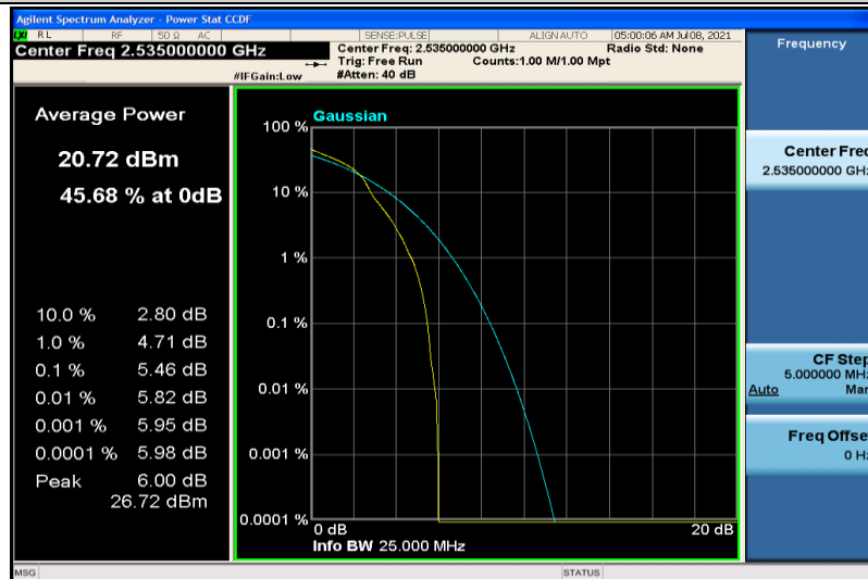
Band7-10MHz-16QAM-21100-1RB#0
