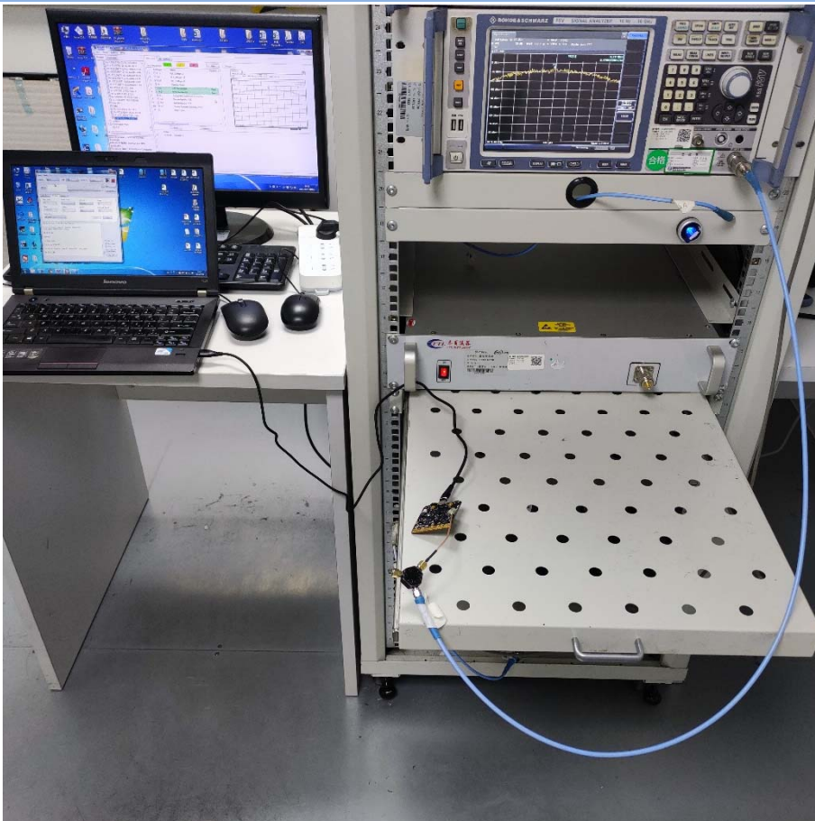
Conducted Test
