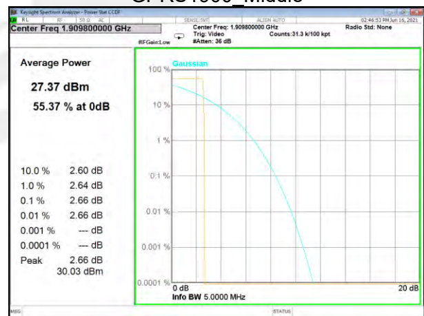
GPRS1900_Higher
