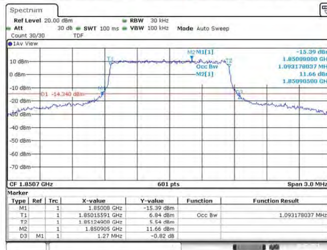
Band2-1.4MHz-QPSK-18607-6RB#0-1.093
