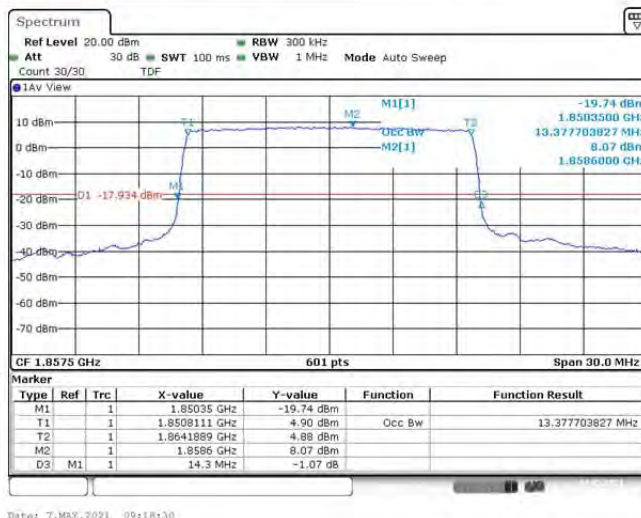
Band2-15MHz-QPSK-18900-75RB#0-13.378
