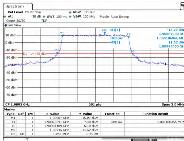
Band2-1.4MHz-QPSK-19193-6RB#0-1.088
