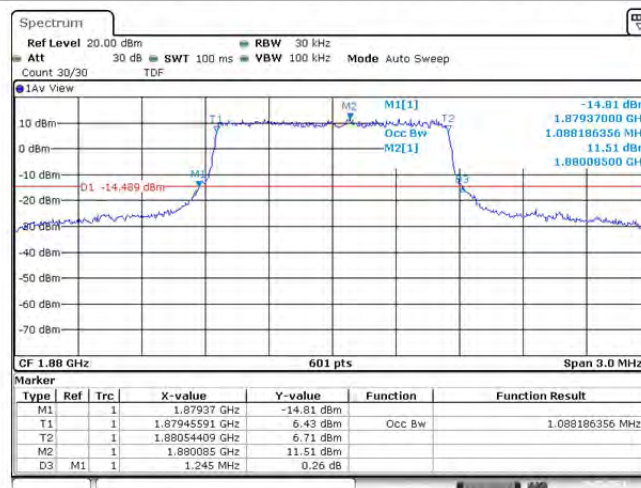
Band2-1.4MHz-QPSK-18900-6RB#0-1.088
