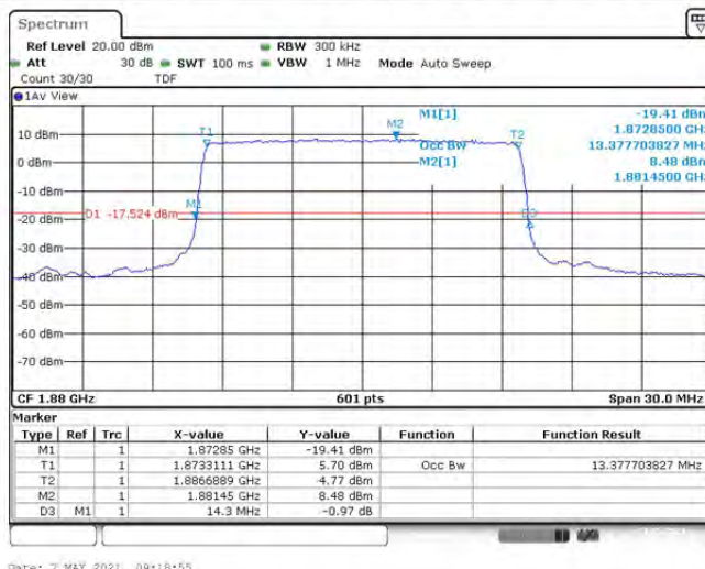
Band2-15MHz-QPSK-19125-75RB#0-13.378
