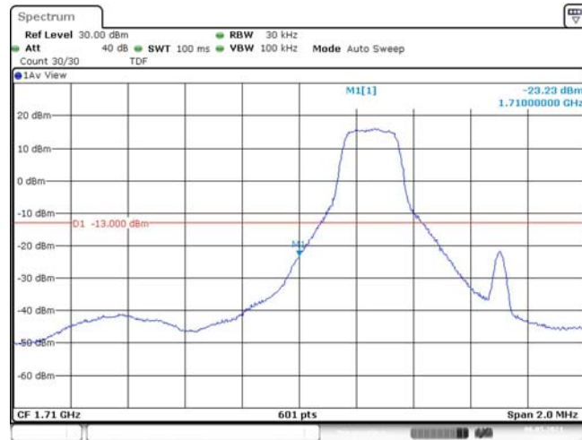
Band4-1.4MHz-QPSK-19957-1RB#0
