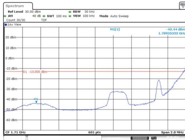
Band4-1.4MHz-QPSK-19957-1RB#5
