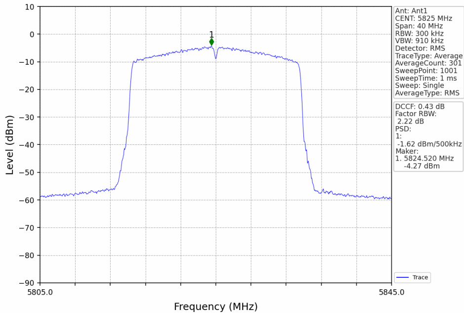
802.11ax(HEW20)_HCH_5825MHz_RU242_Left_Ant1_NTNV
