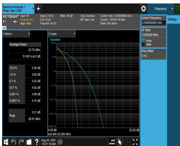
Band7-20MHz-QPSK-21100-100RB#0
