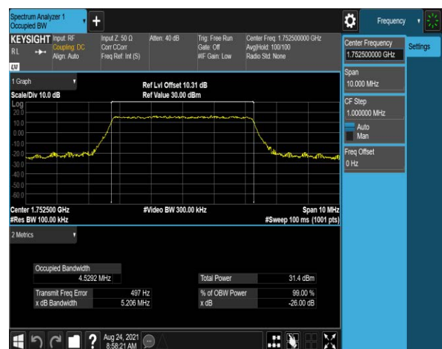
Band4-5MHz-16QAM-20375-25RB#0
