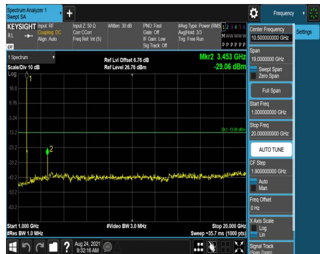
Band4-20MHz-16QAM-20300:1000~20000MHz
