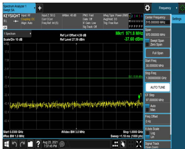
Band2-1.4MHz-QPSK-18900:30~1000MHz
