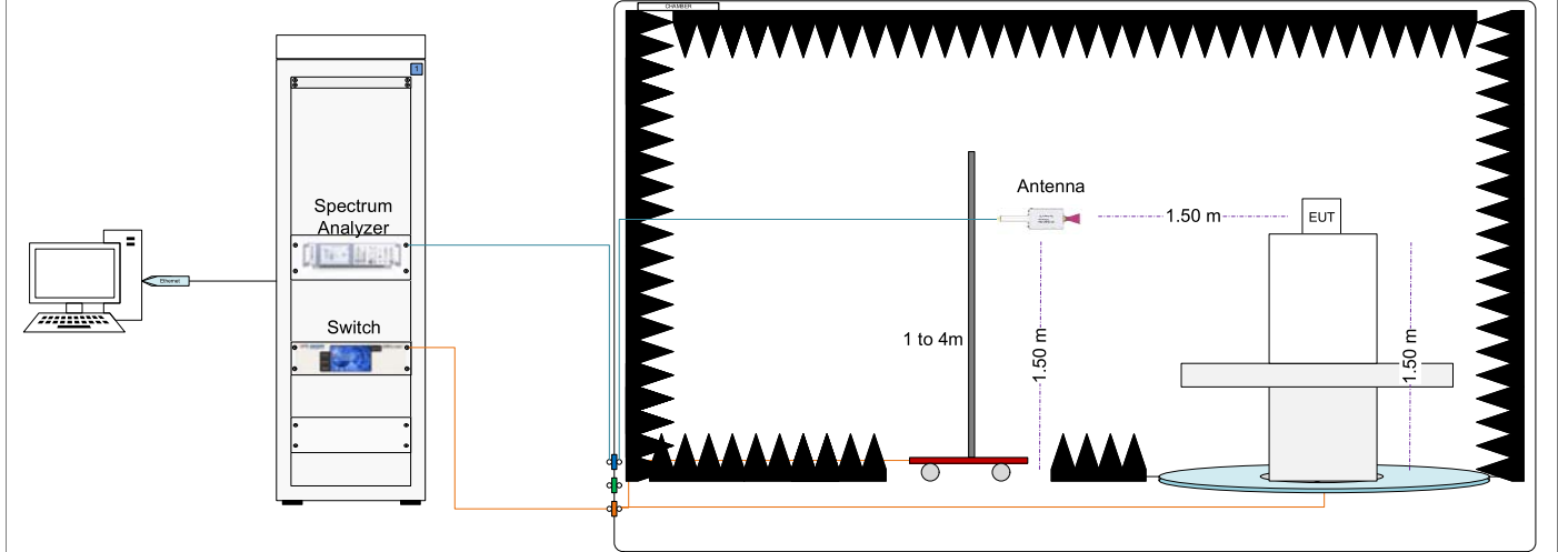
Radiated Setup 18 GHz – 40 GHz (Transmitter tests)
