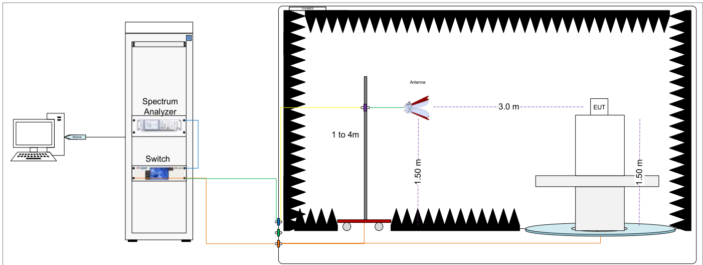
Radiated Setup 9.5 GHz - 18 GHz (Transmitter tests)
