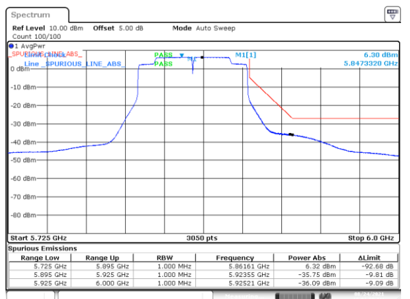
BE-NR-HIGH, SISO-A, 802.11ac80-VHT0, Ch171
