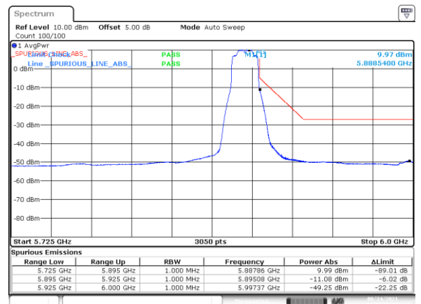
BE-NR-HIGH, MIMO-B, 802.11n20-HT8, Ch177
