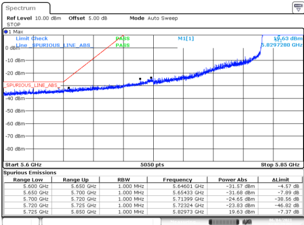
BE-NR-LOW, SISO-B, 802.11ax80-HE0, Ch171
