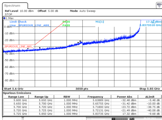
BE-NR-LOW, MIMO-A, 802.11ac80-VHT0, Ch171
