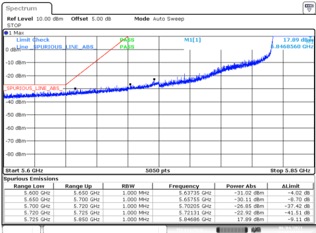
BE-NR-LOW, SISO-B, 802.11ac80-VHT0, Ch171
