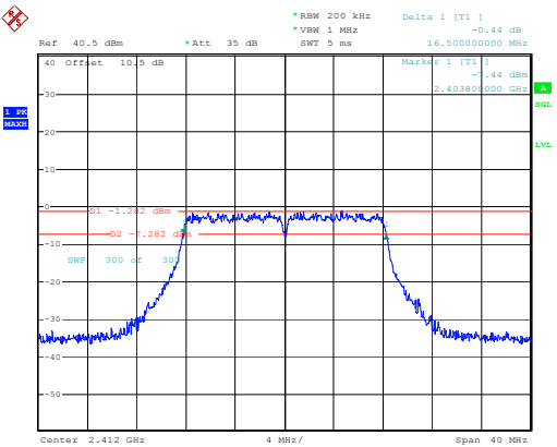
802.11g_2412MHz
