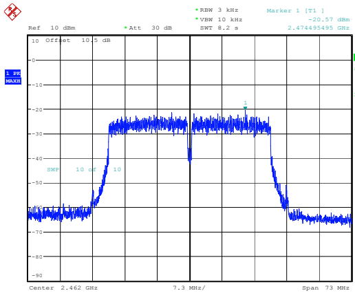
802.11n40_2462MHz
