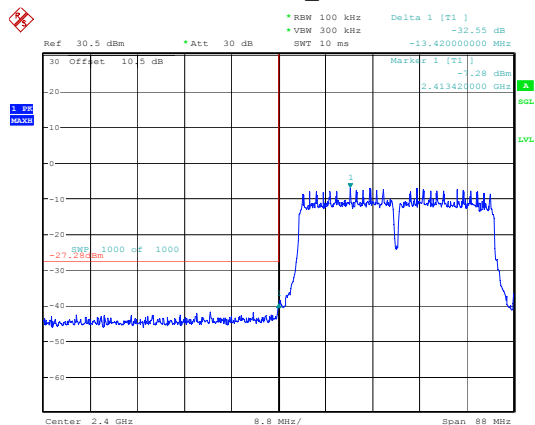
802.11n40_2422MHz
