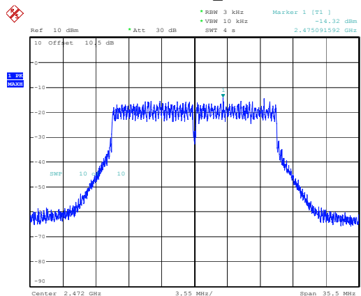
802.11n20_2472MHz
