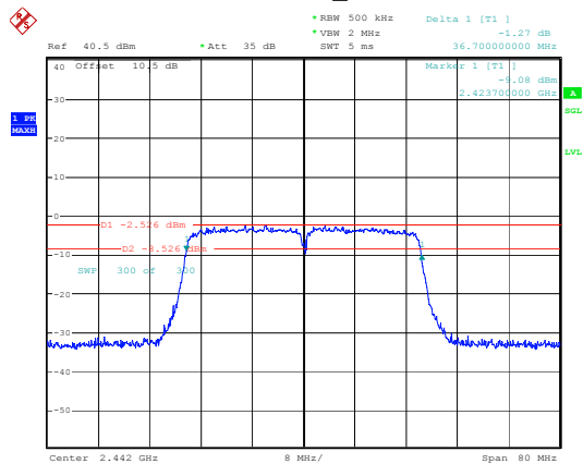
802.11n40_2442MHz
