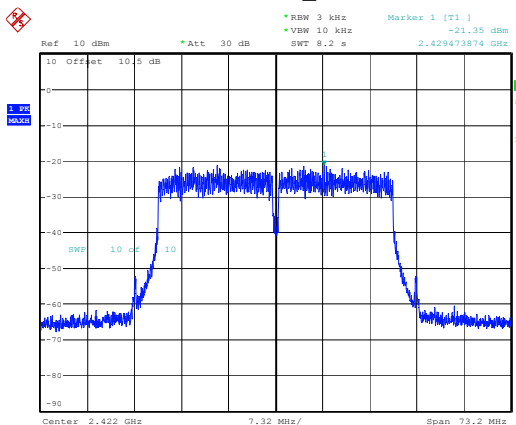
802.11n40_2422MHz
