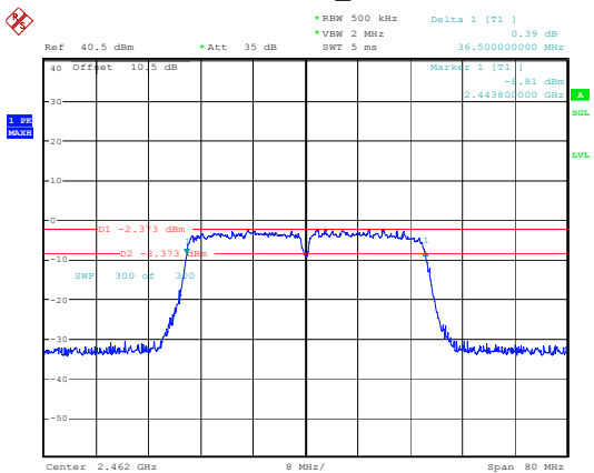
802.11n40_2462MHz
