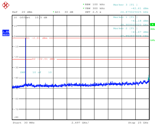
802.11g_2442MHz
