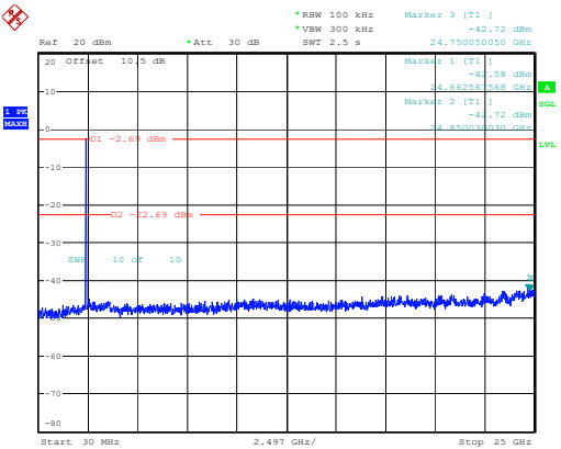
802.11g_2412MHz
