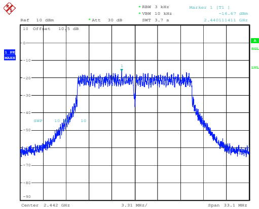
802.11g_2442MHz
