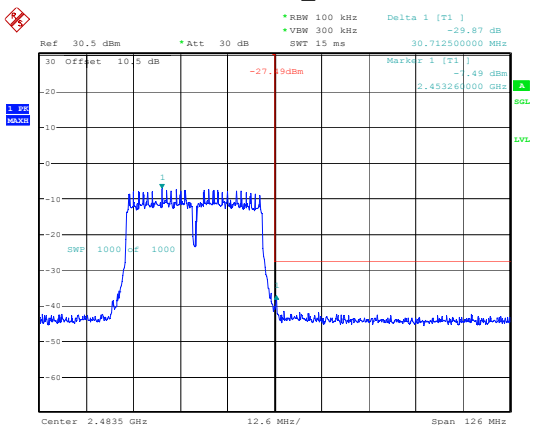
802.11n40_2462MHz
