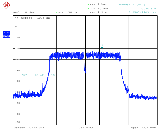
802.11n40_2442MHz
