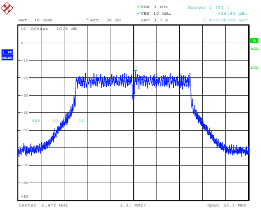
802.11g_2472MHz
