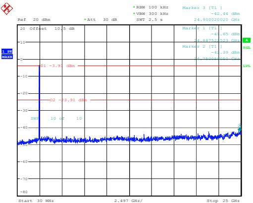
802.11g_2472MHz
