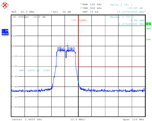
802.11n20_2472MHz
