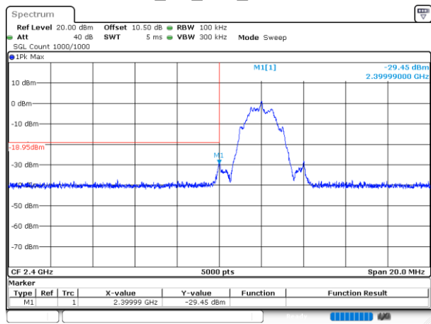
BLE_2M_Low_Channel
