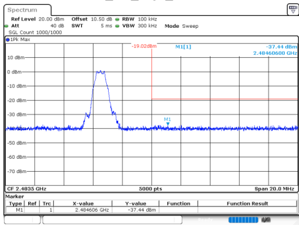
BLE_1M_High_Channel
