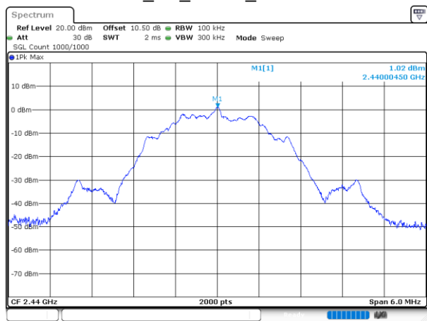
BLE_2M_Middle_Channel
