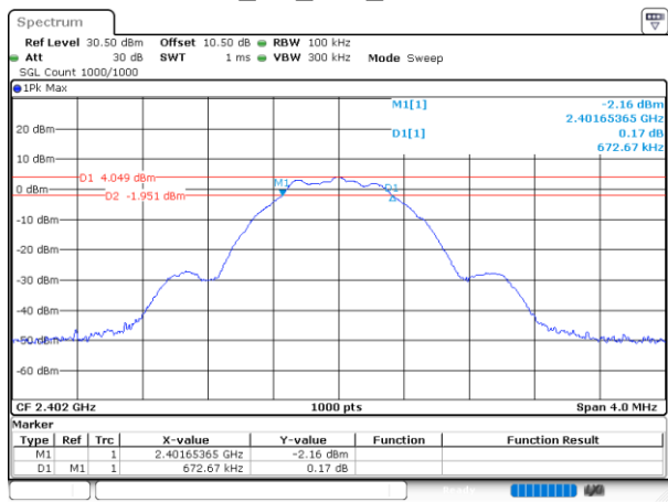
BLE_1M_Low_Channel
