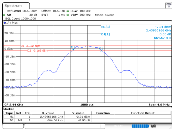
BLE_1M_Middle_Channel
