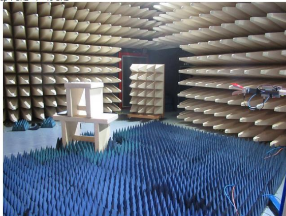
Test Setup f > 18 \text{ GHz}
