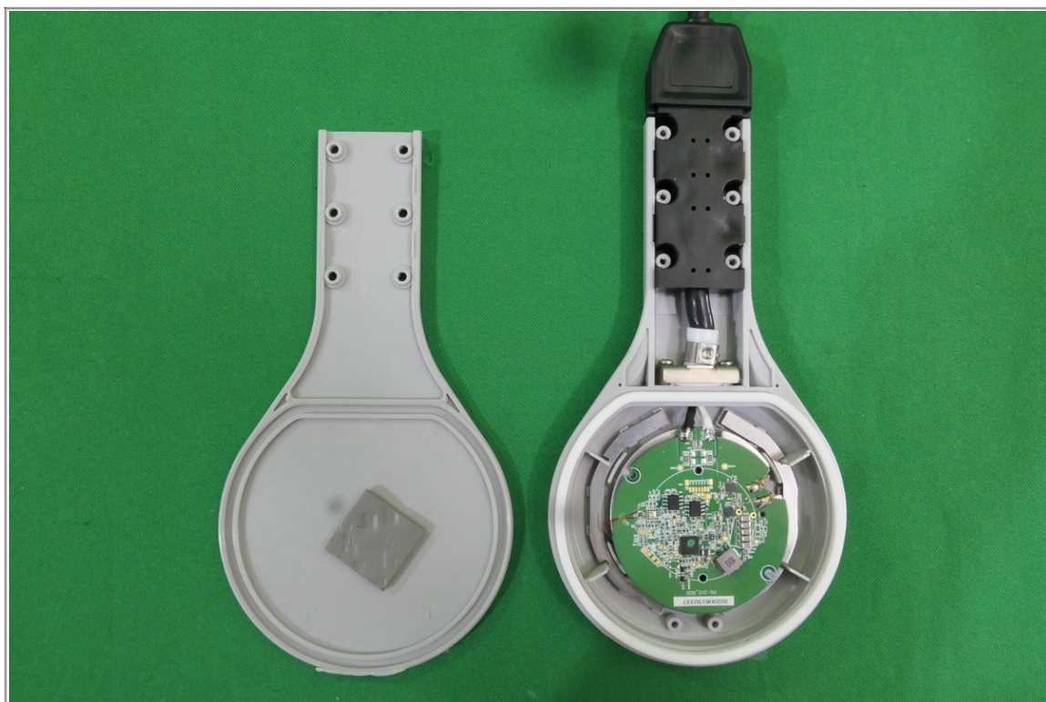
Inner View of EUT-1
