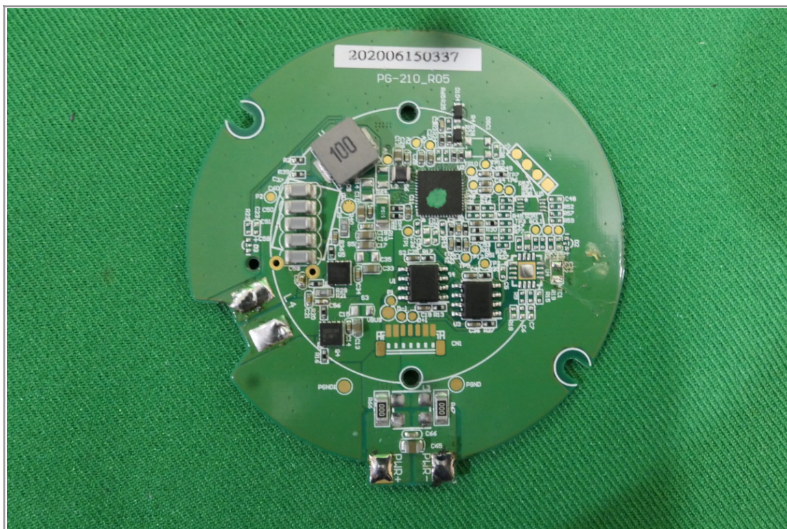
Component View of PCBA-1
