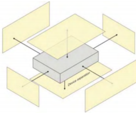
Figure 7.1 – Test positions for generic device
