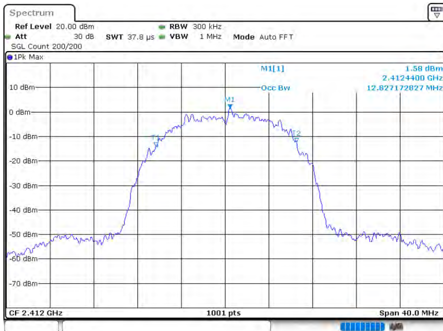
OBW NVNT 802.11b 2412MHz Ant3
