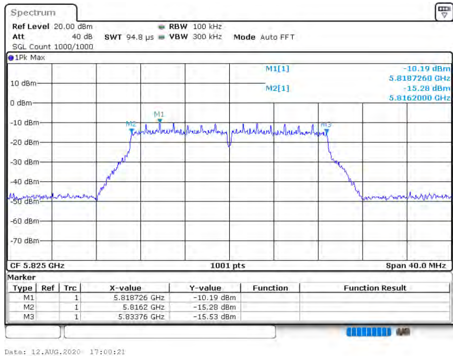
EBW NVNT 802.11n(HT20) 5825MHz Ant 2
