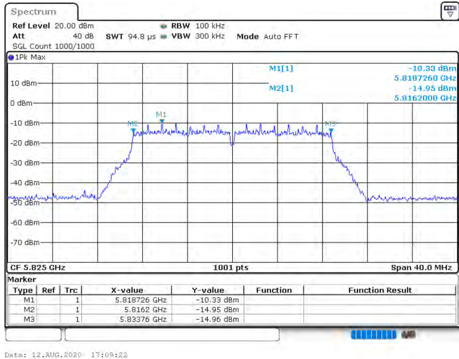
EBW NVNT 802.11ac20 5825MHz Ant 2
