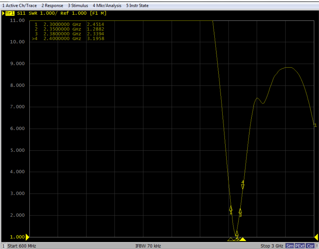
S11-SWR
