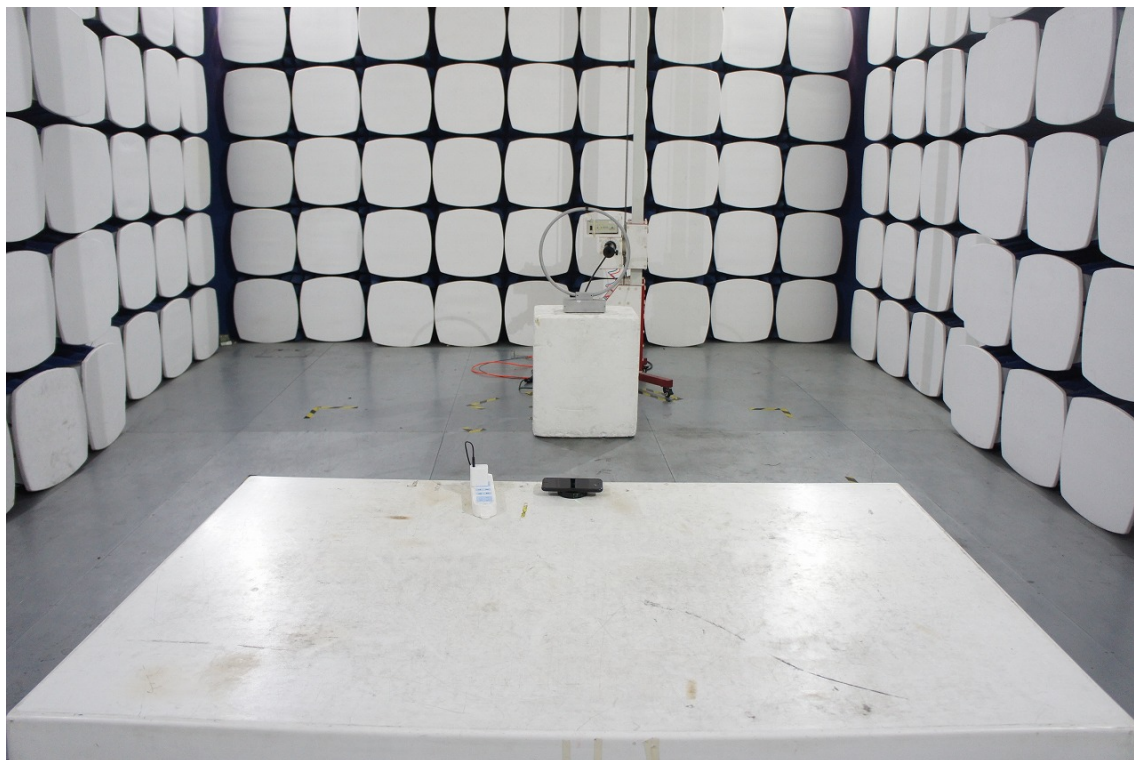
Radiated Setup photo (Below 30MHz)
