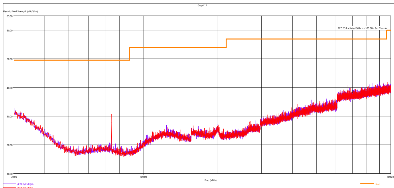
Figure 8 - Radiated Emissions Plot, 30 MHz-1 GHz, Receive Mode
