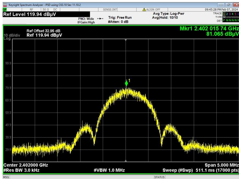
Figure 21 – EIRP Power Spectral Density, Low Channel Corrected values measured at 3m.
