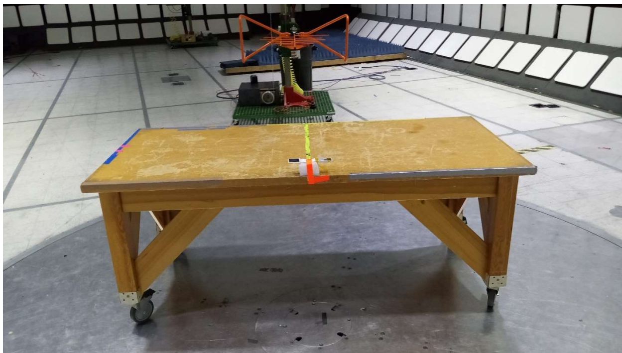
Setup, 30MHz – 1GHz
