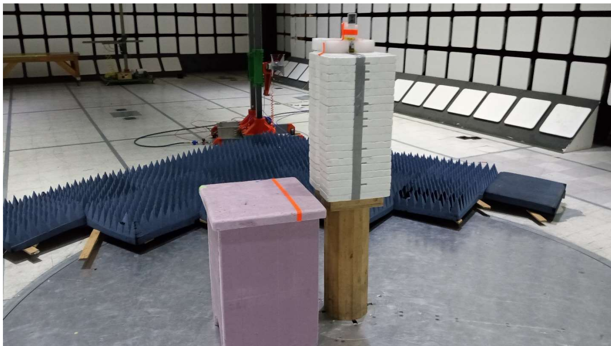
Setup, 1GHz – 18GHz
