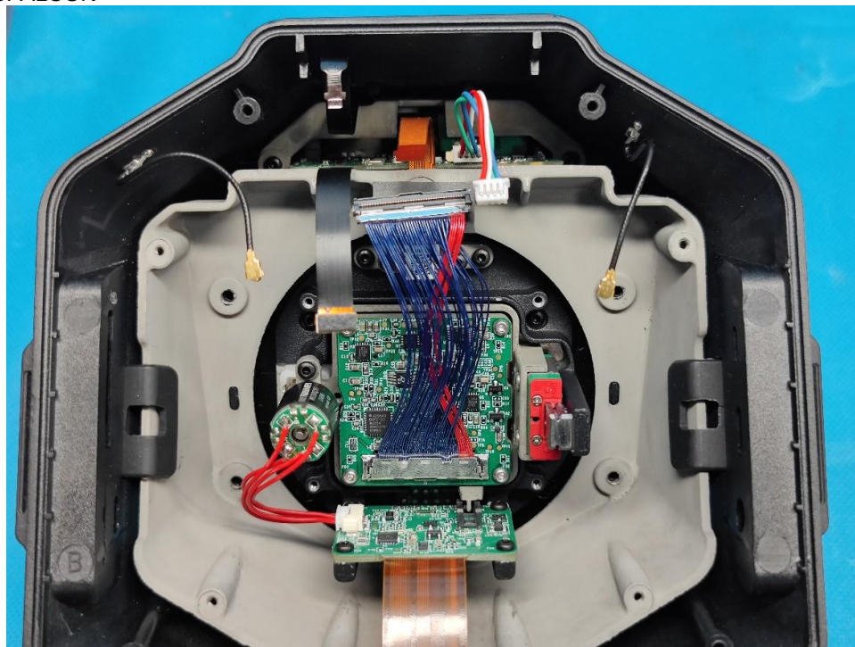
Wi-Fi and Bluetooth Antenna
