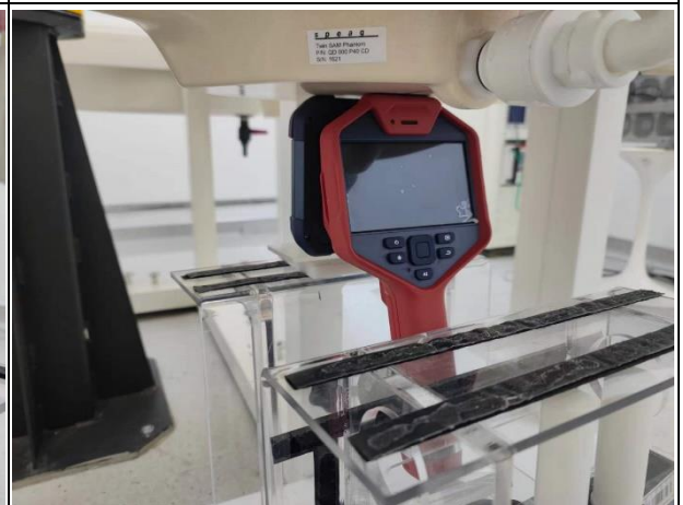
Figure 1.1-6 Top side 0mm
