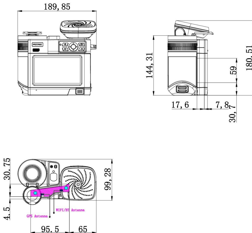
Figure 12.2-1 Antenna Locations
