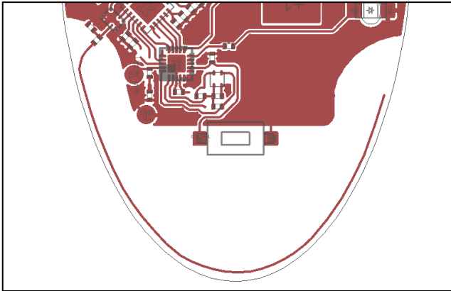
Single wire antenna as PCB print
