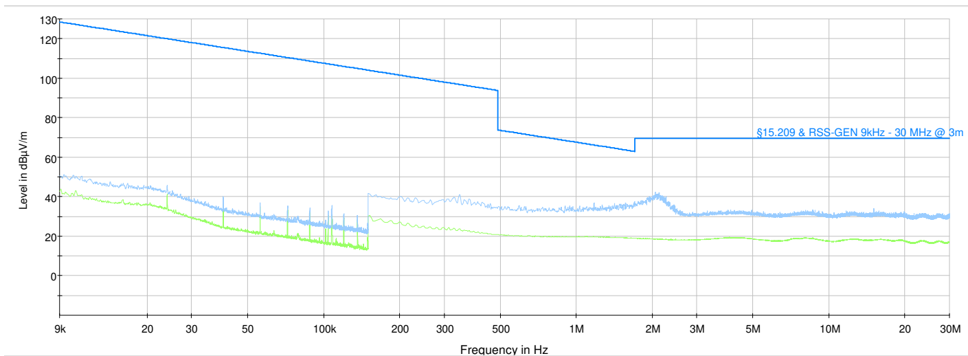
Preliminary test results from 9 kHz to 30 MHz
