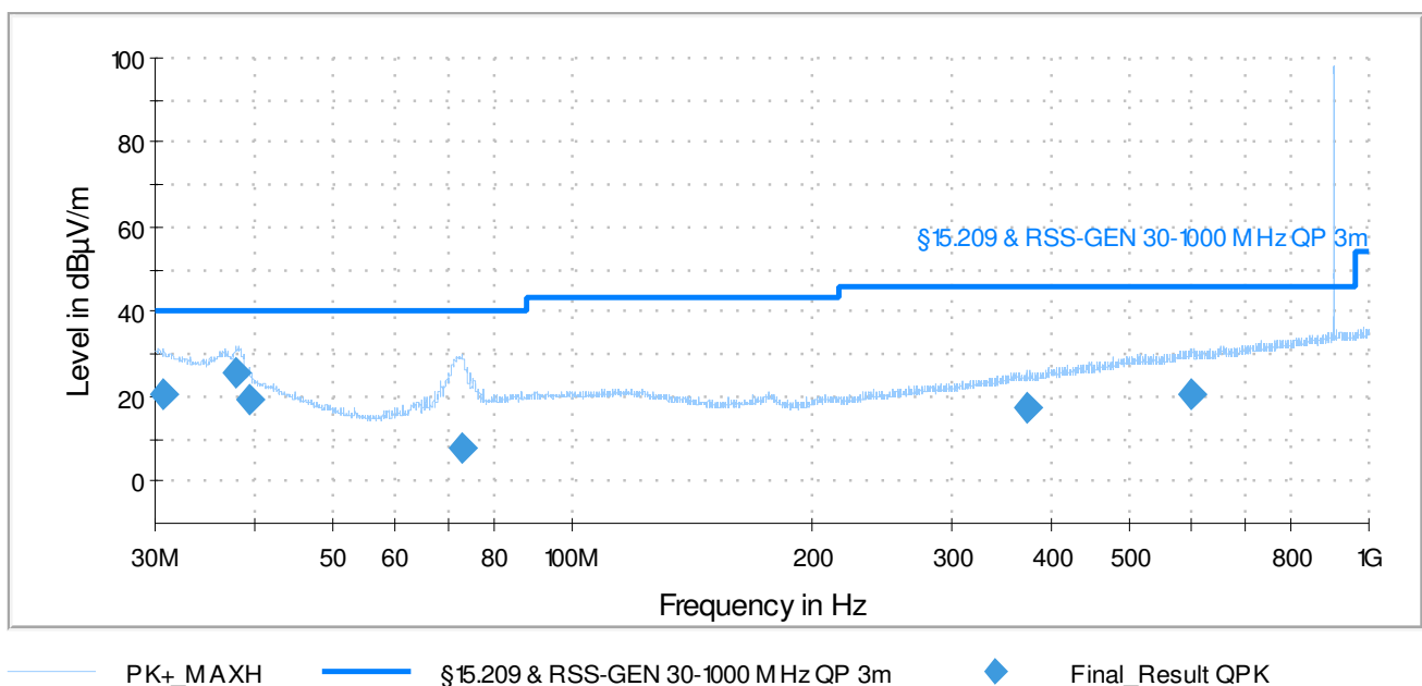
Final test results from 30 MHz to 1 GHz
