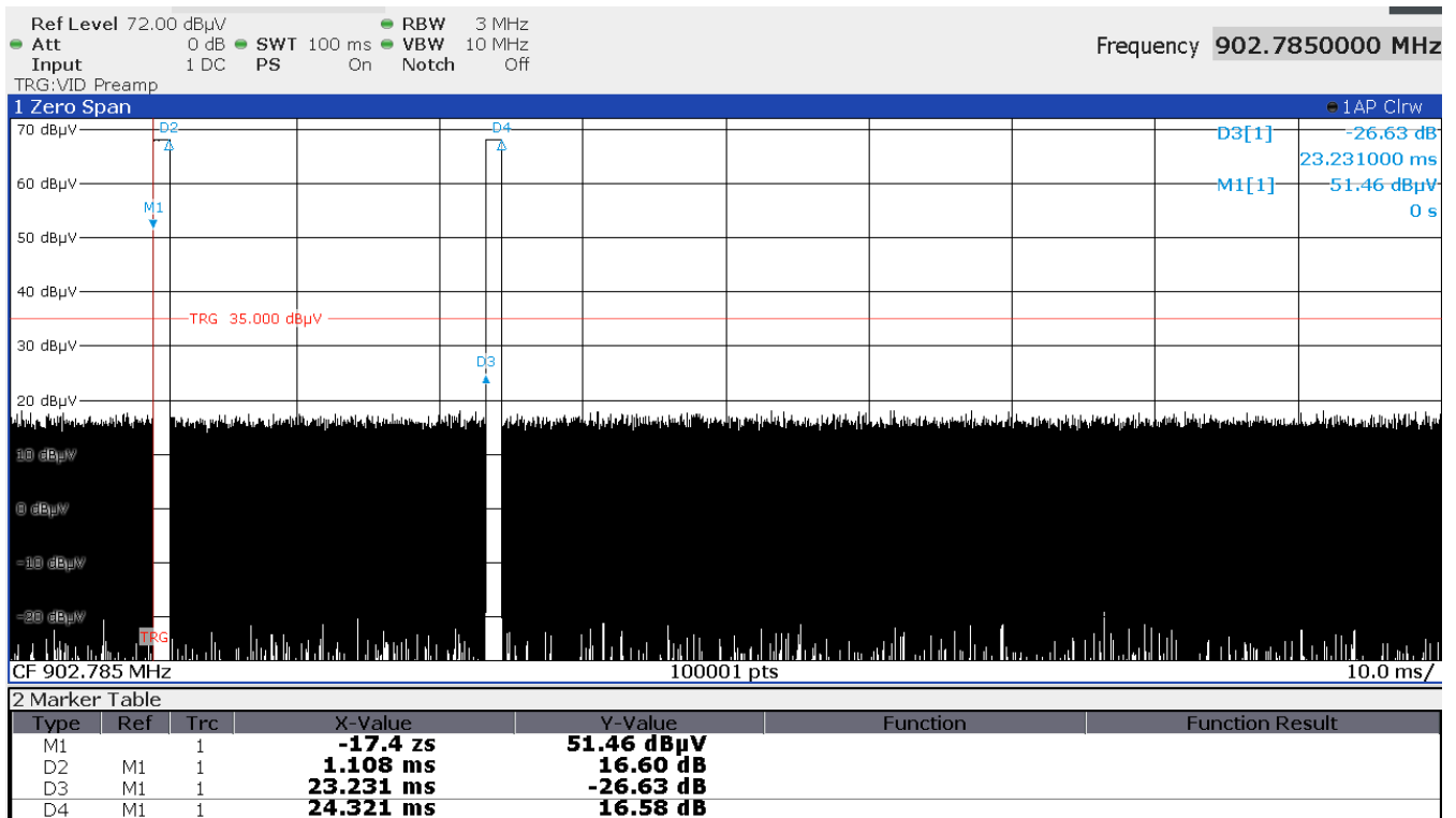
Plot showing pulse transmission time
