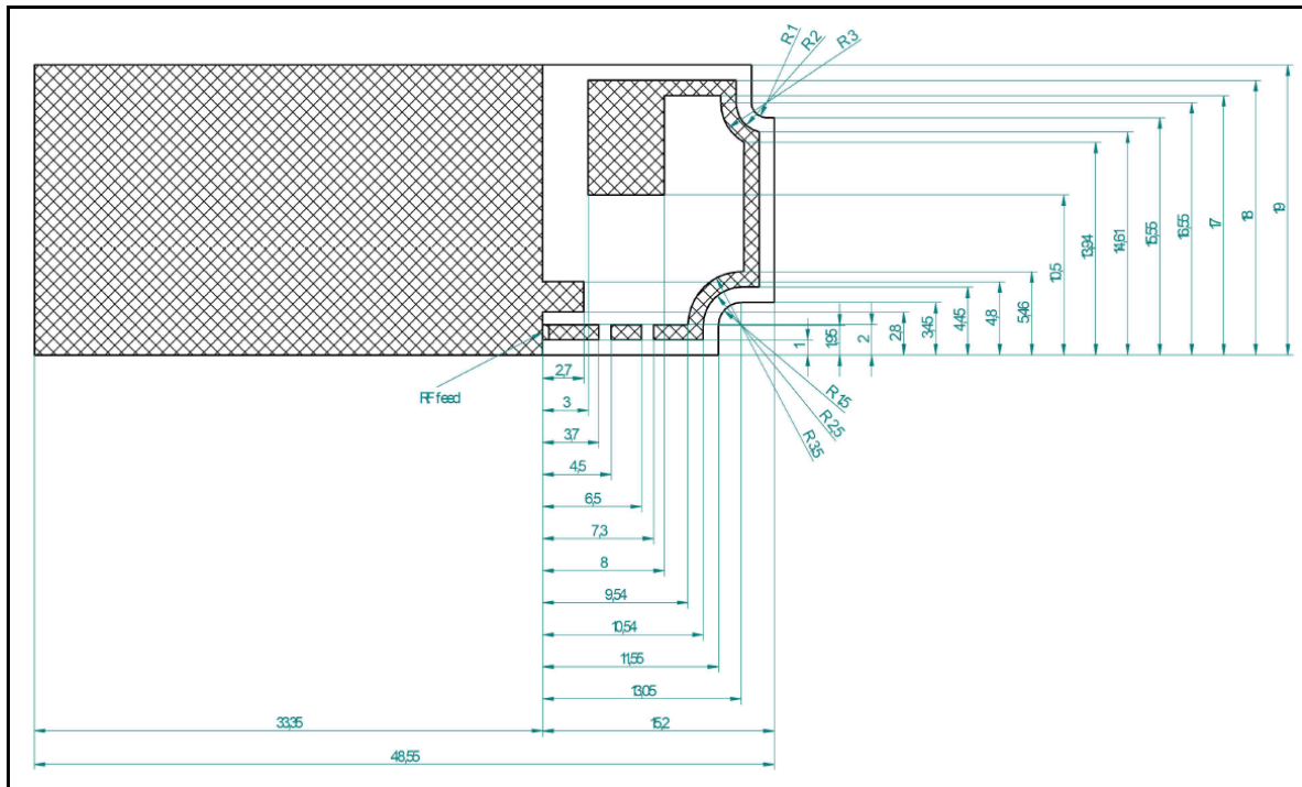
Antenna drawing "ANT_PCB_436_01":
