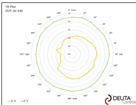
Antenna pattern "ANT_PCB_436_01"
