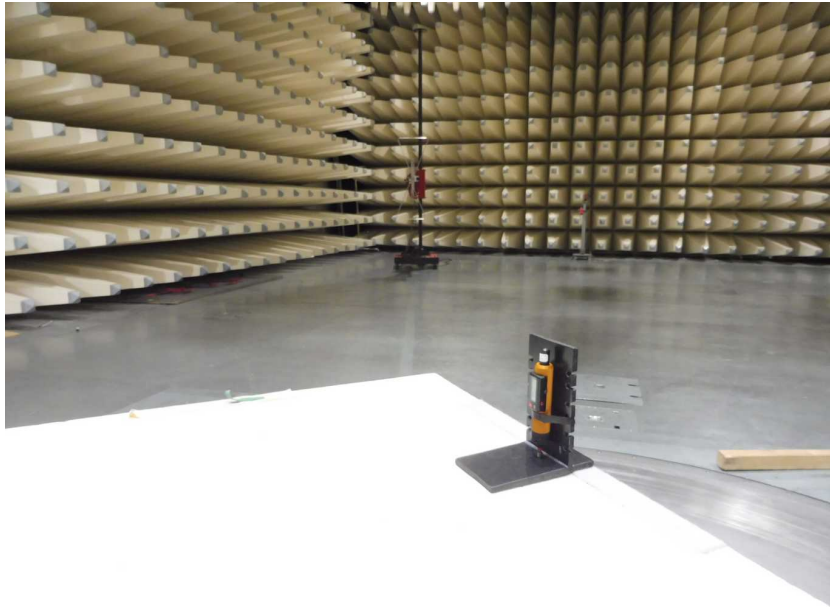
Photo 7: EUT at the semi-anechoic chamber
