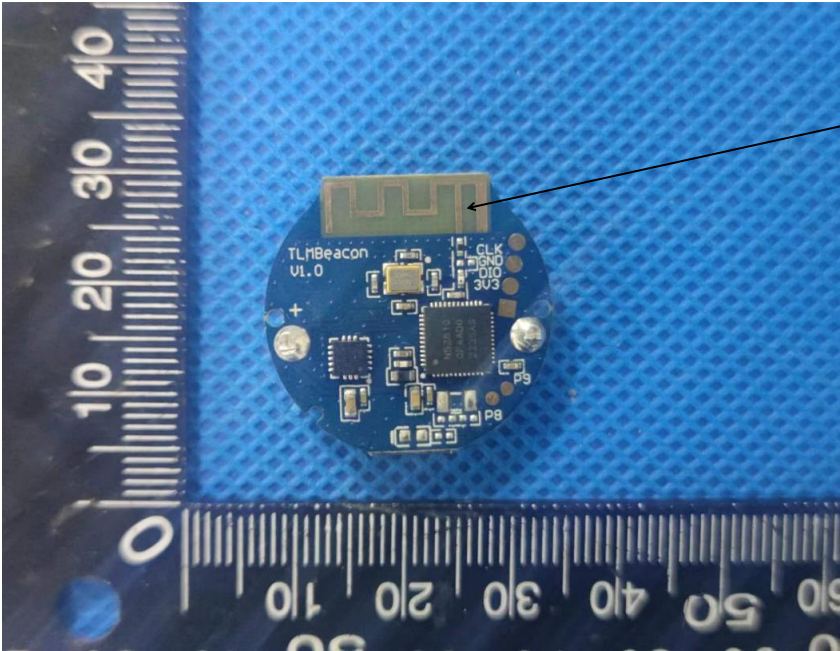
PCB Antenna
