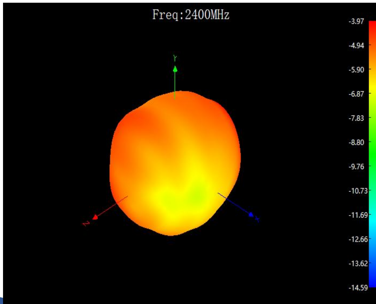
3D-Etotal (2400Mhz)
