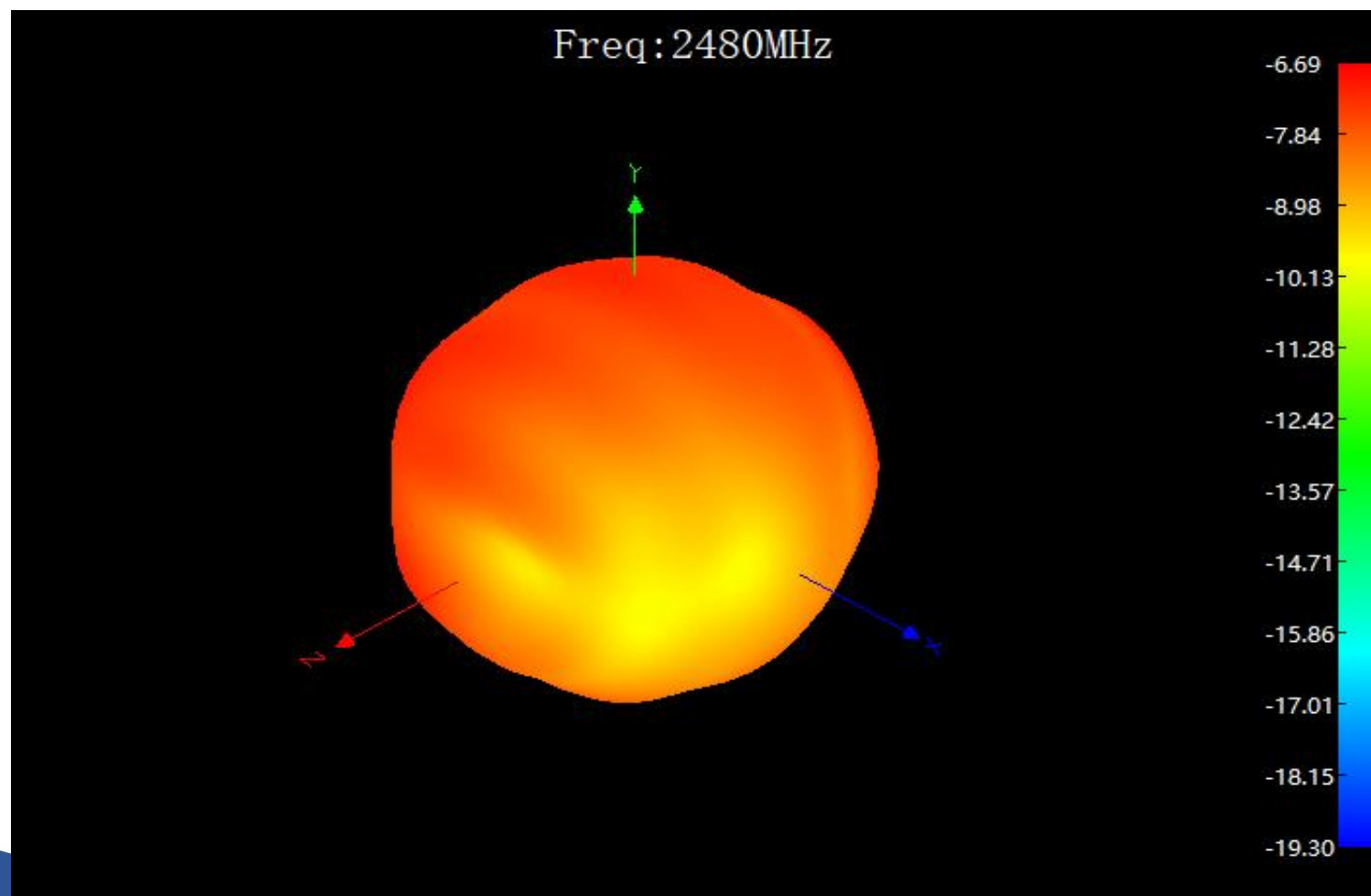
3D-Etotal (2480Mhz)
