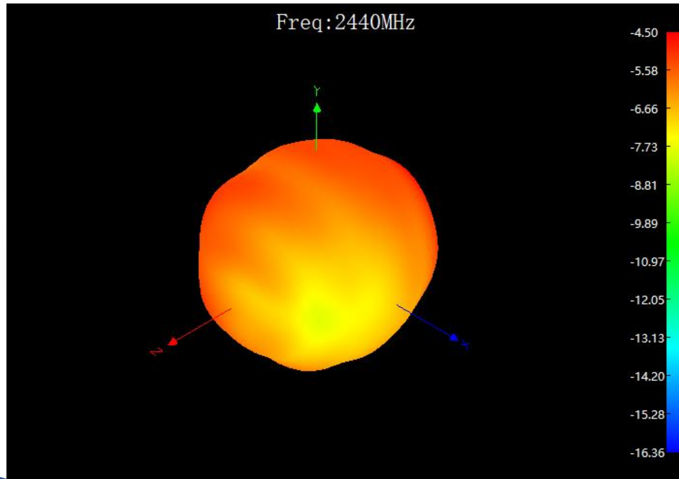
3D-Etotal (2440Mhz)
