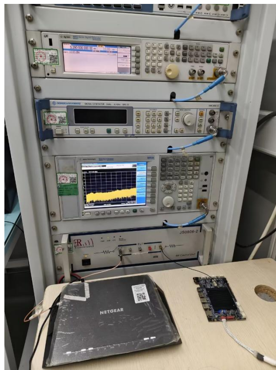
DFS test setup
