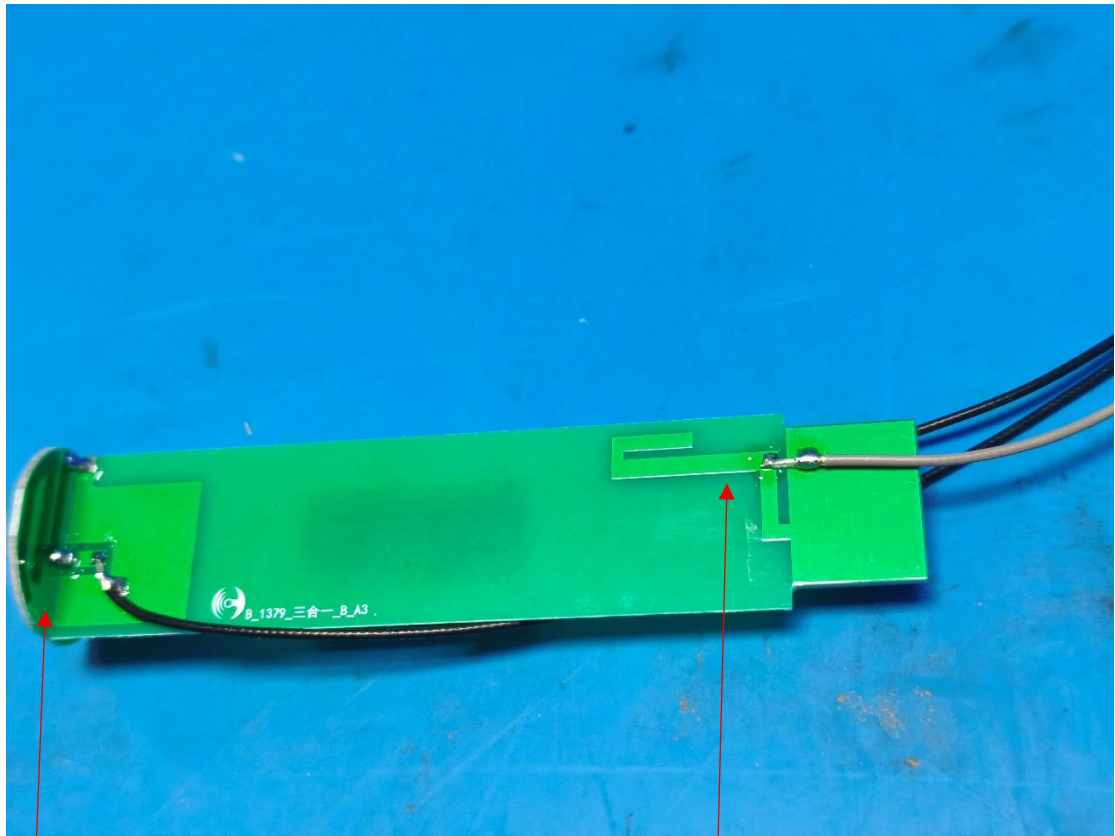
WiFi antenna 1
