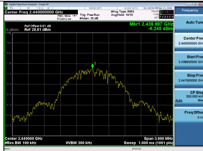
BLE_1M-Ant1-2440-0~Reference-PASS
