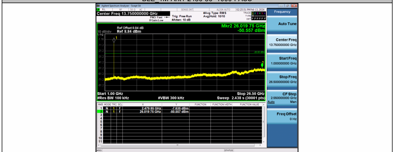
BLE_1M-Ant1-2480-1000~26500-PASS
