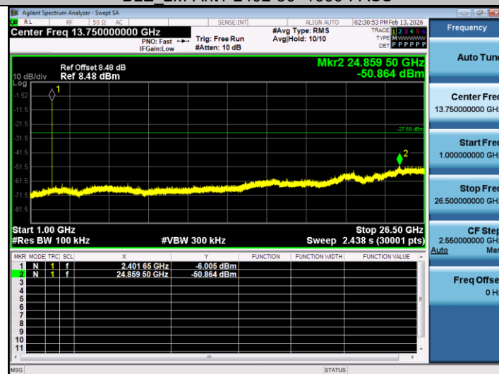
BLE_2M-Ant1-2402-1000~26500-PASS
