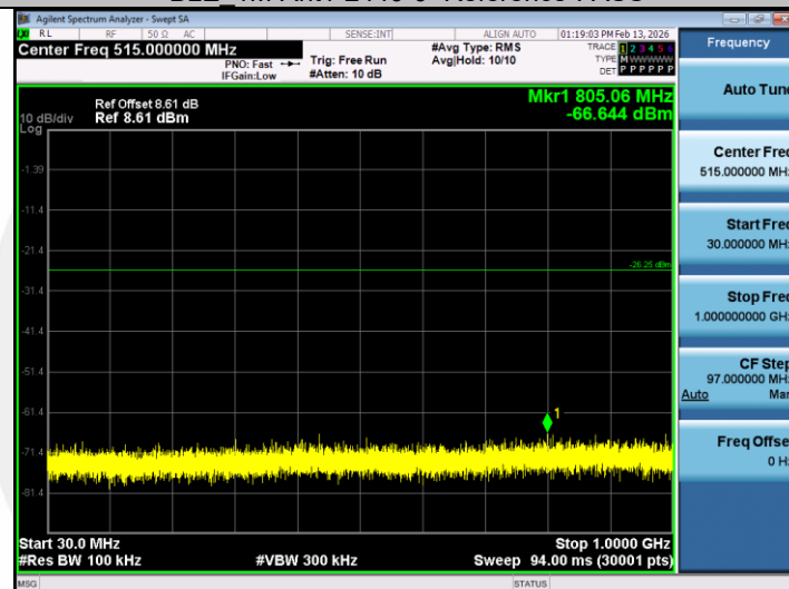
BLE_1M-Ant1-2440-30~1000-PASS
