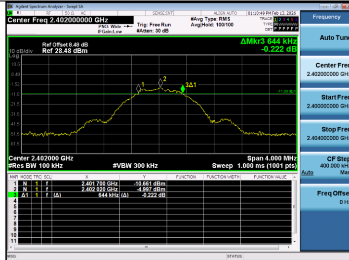
BLE_1M-Ant1-2402-PASS
