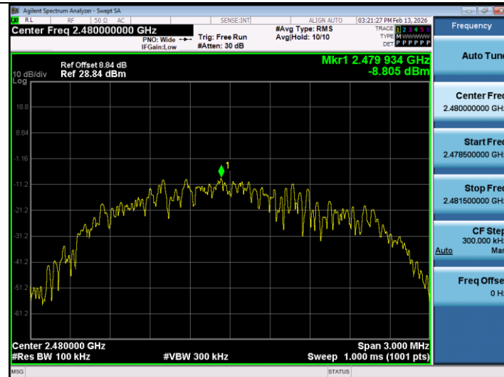
BLE_2M-Ant1-2480-0~Reference-PASS
