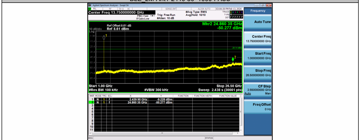
BLE_2M-Ant1-2440-1000~26500-PASS
