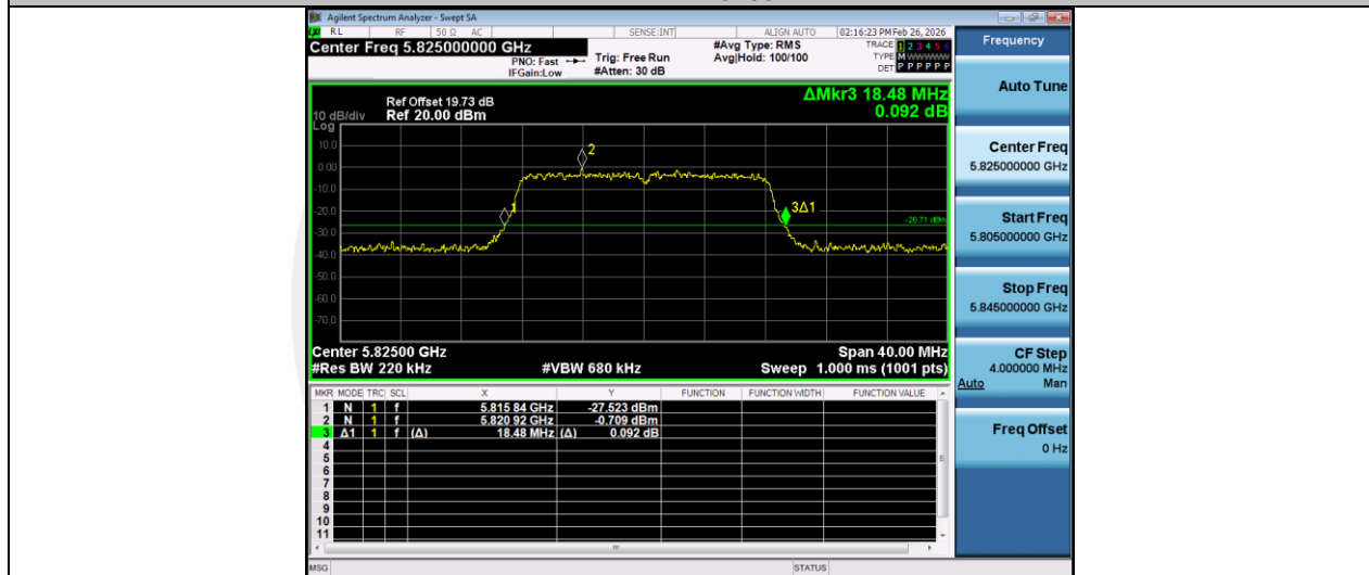
11A-Ant1-5825
