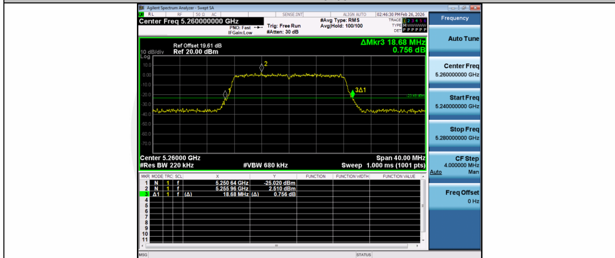
11A-Ant2-5260
