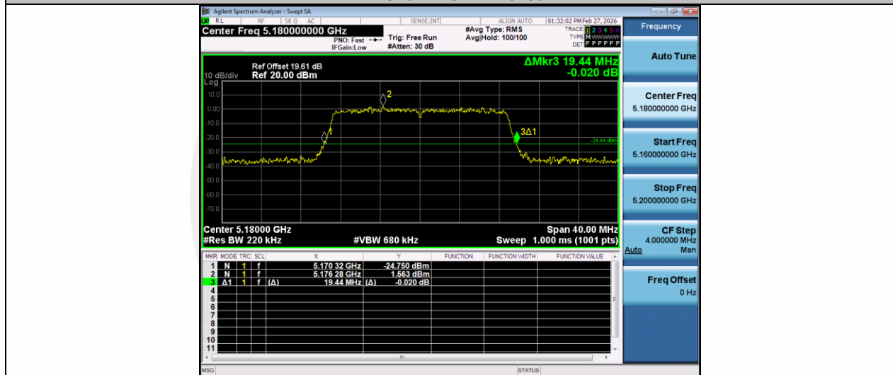
11AC20MIMO-Ant2-5180
