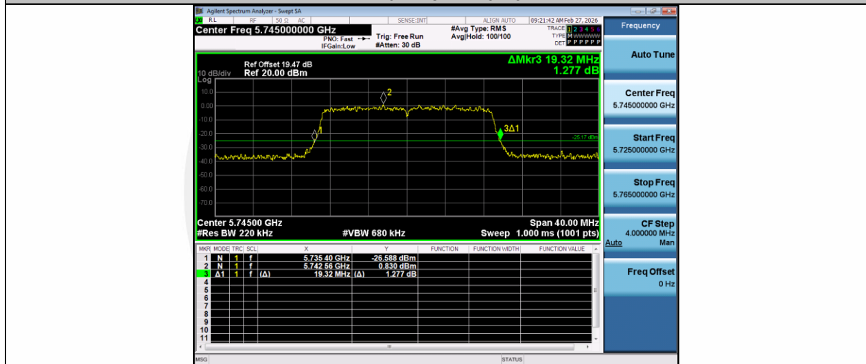
11N20MIMO-Ant2-5745
