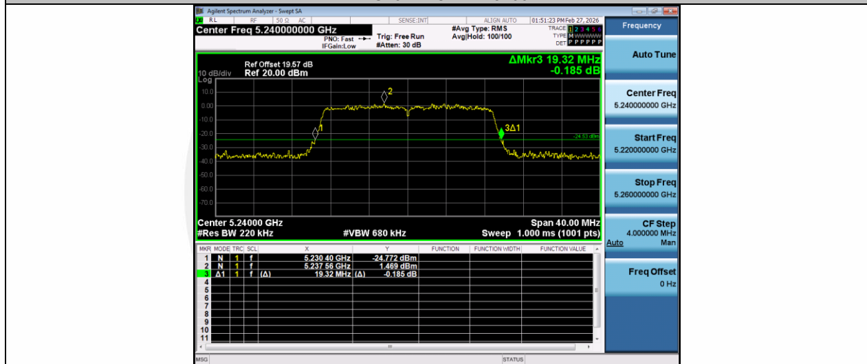
11AC20MIMO-Ant1-5240
