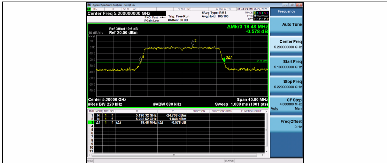
11AC20MIMO-Ant2-5200
