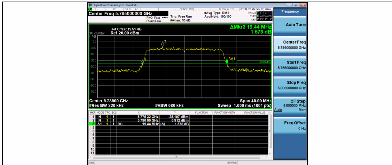
11AC20MIMO-Ant2-5785
