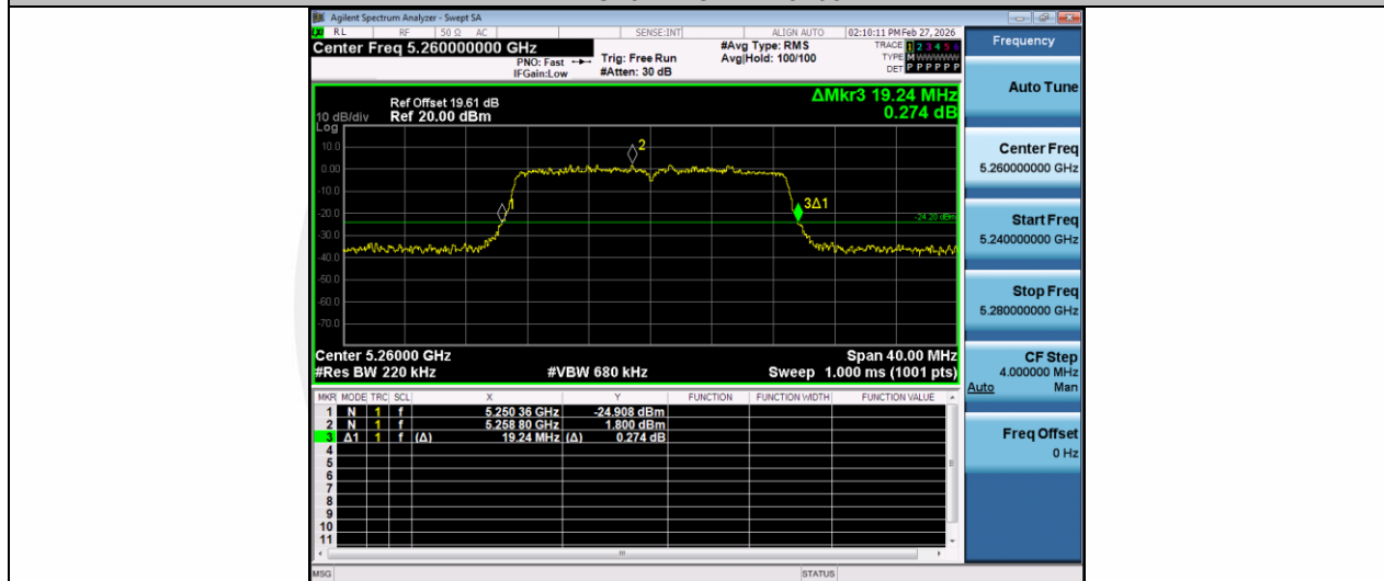
11AC20MIMO-Ant2-5260
