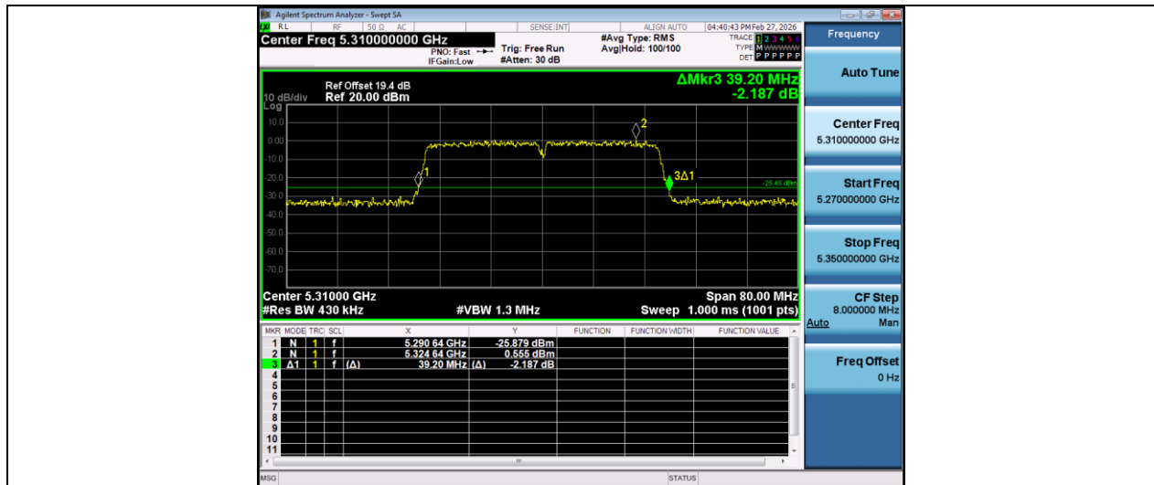
11AC40MIMO-Ant1-5310
