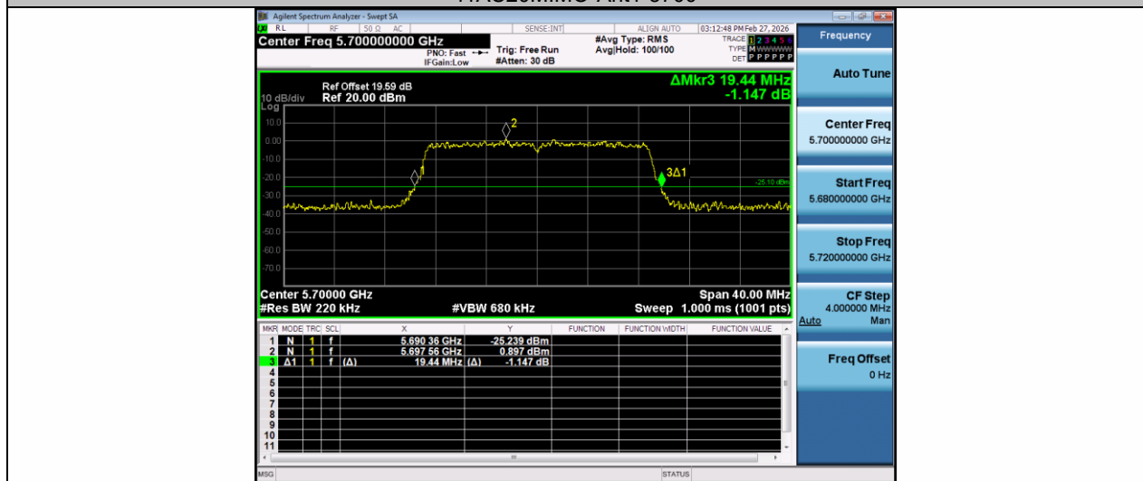
11AC20MIMO-Ant2-5700
