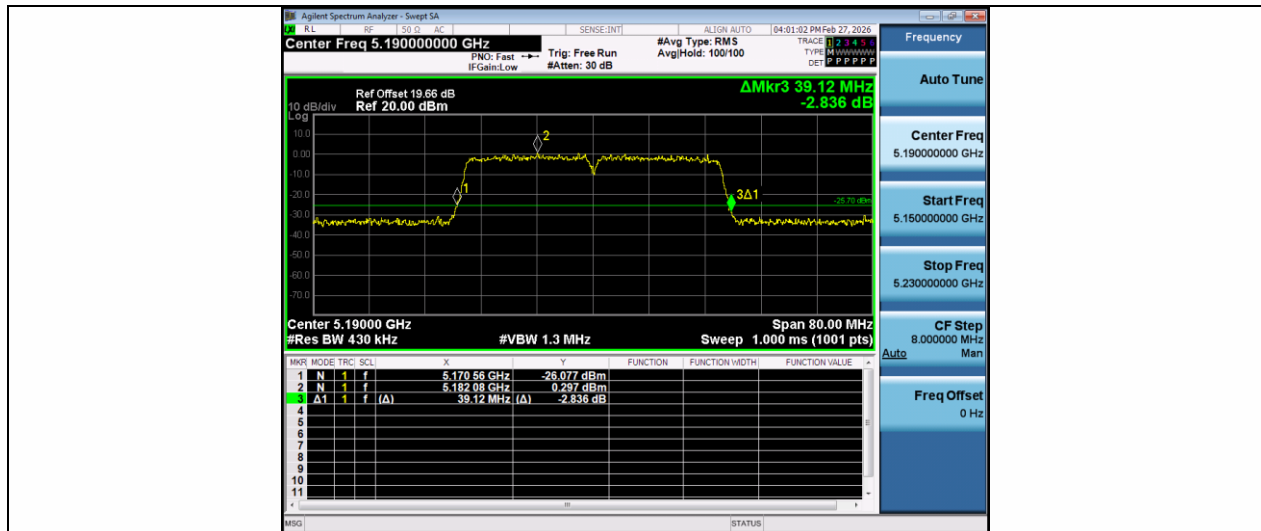
11AC40MIMO-Ant1-5190
