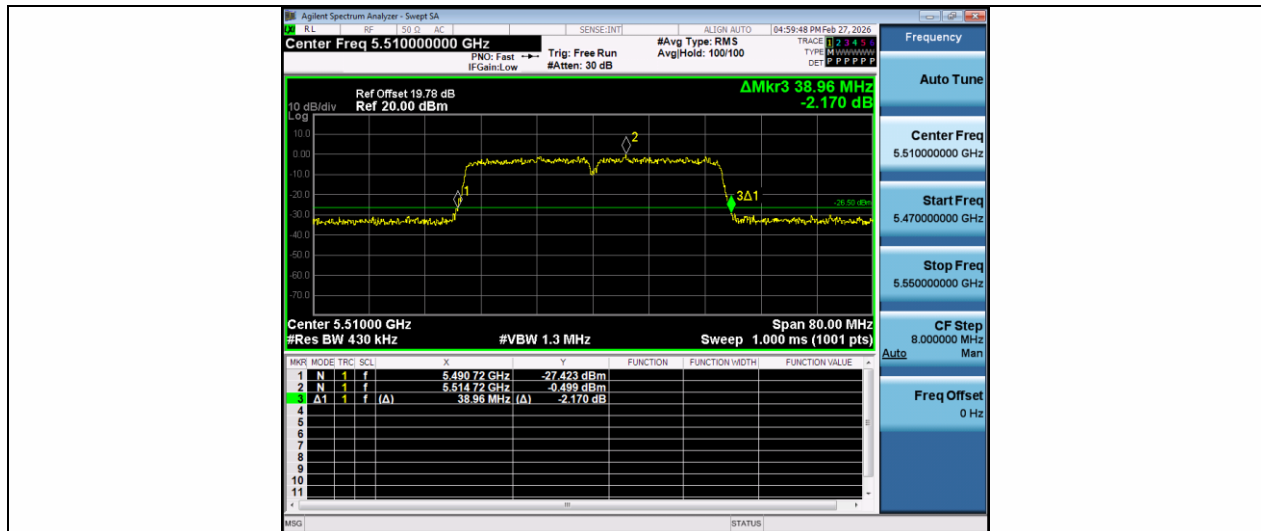
11AC40MIMO-Ant2-5510
