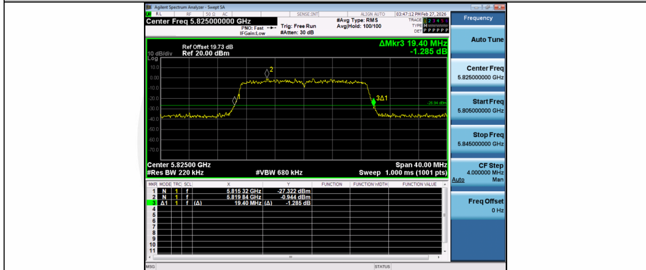
11AC20MIMO-Ant1-5825
