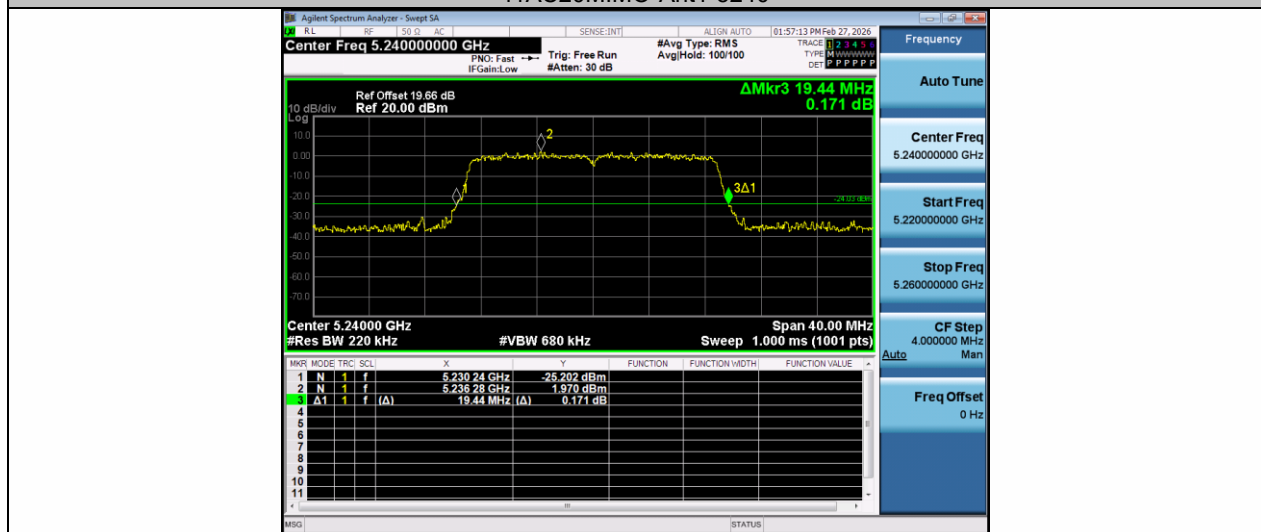
11AC20MIMO-Ant2-5240
