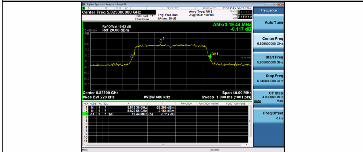
11AC20MIMO-Ant2-5825
