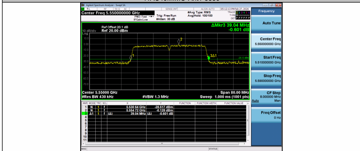
11AC40MIMO-Ant2-5550
