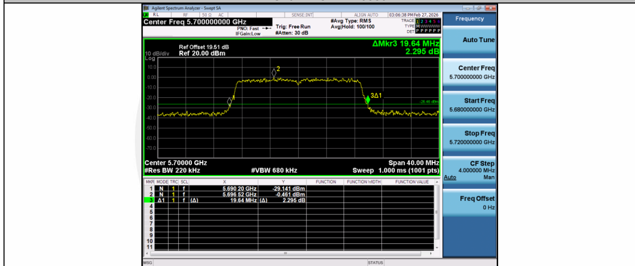
11AC20MIMO-Ant1-5700
