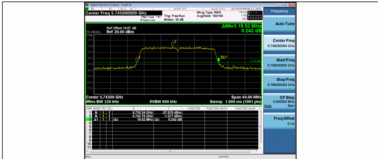
11AC20MIMO-Ant1-5745
