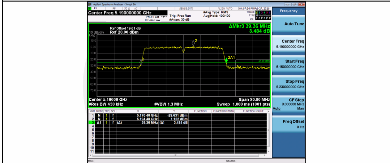
11AC40MIMO-Ant2-5190
