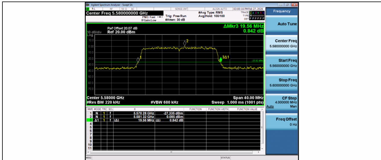
11AC20MIMO-Ant2-5580
