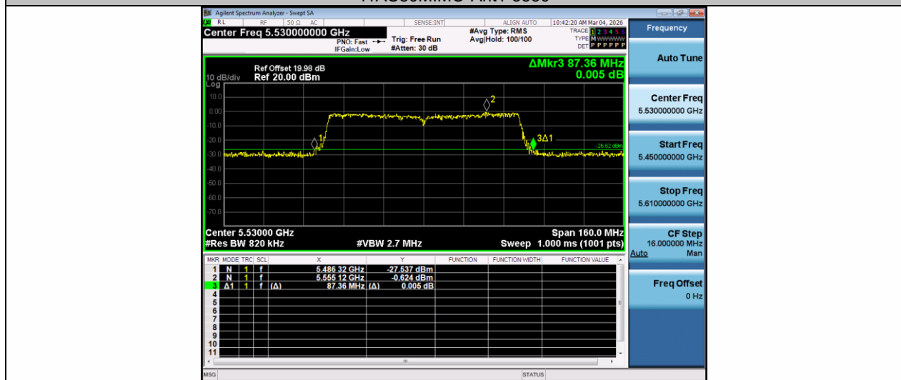
11AC80MIMO-Ant2-5530
