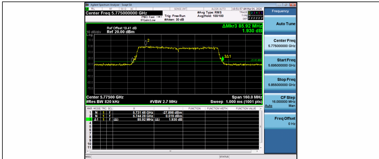
11AC80MIMO-Ant2-5775
