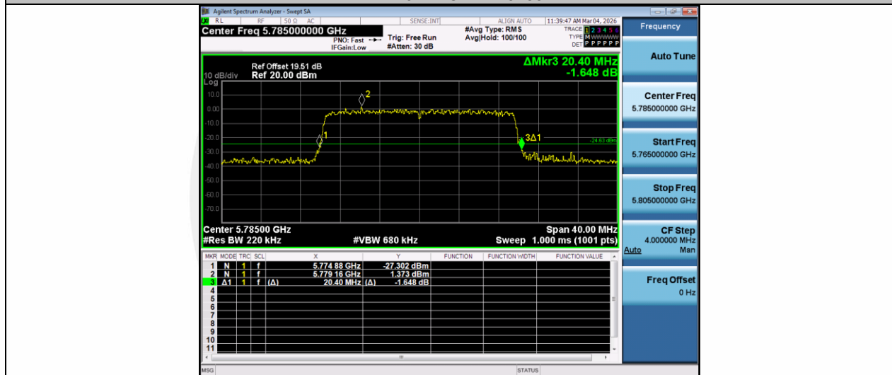
11AX20MIMO-Ant2-5785
