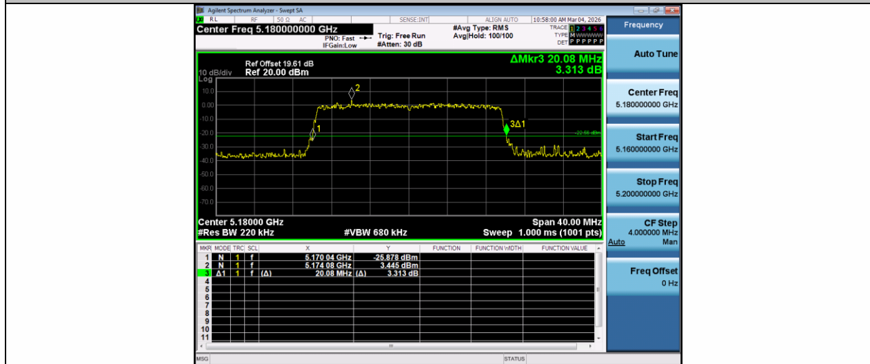
11AX20MIMO-Ant2-5180
