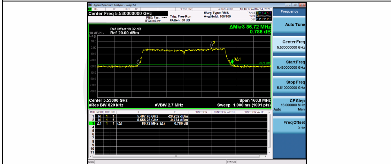
11AC80MIMO-Ant1-5530
