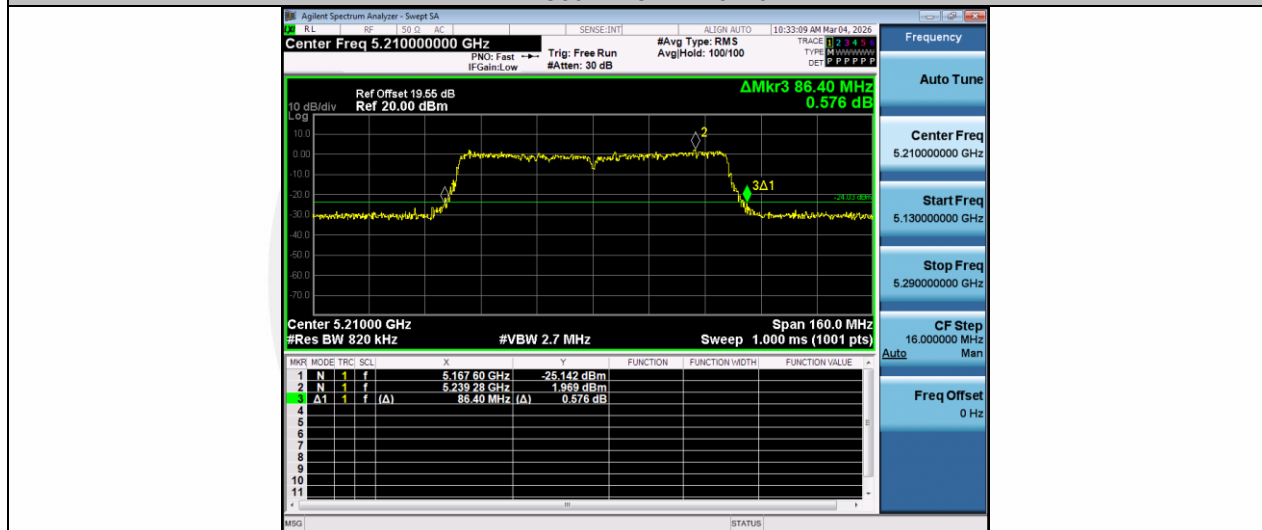
11AC80MIMO-Ant2-5210
