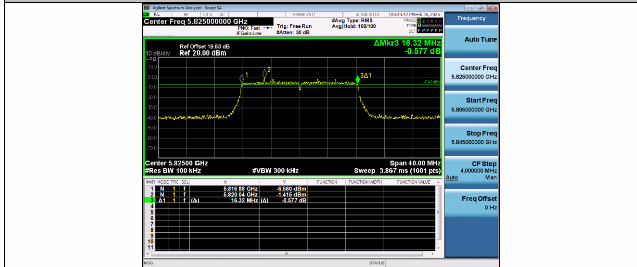
11A-Ant2-5825-PASS
