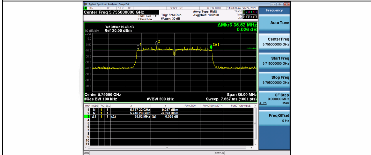
11N40MIMO-Ant2-5755-PASS
