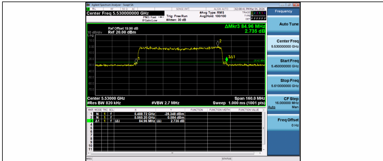
11AX80MIMO-Ant2-5530
