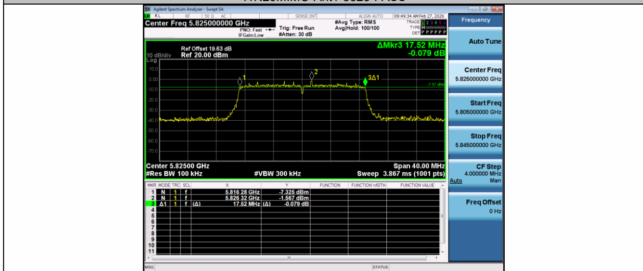
11N20MIMO-Ant2-5825-PASS
