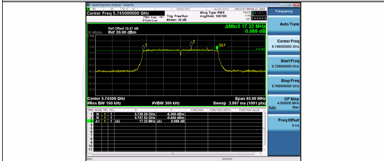
11N20MIMO-Ant2-5745-PASS
