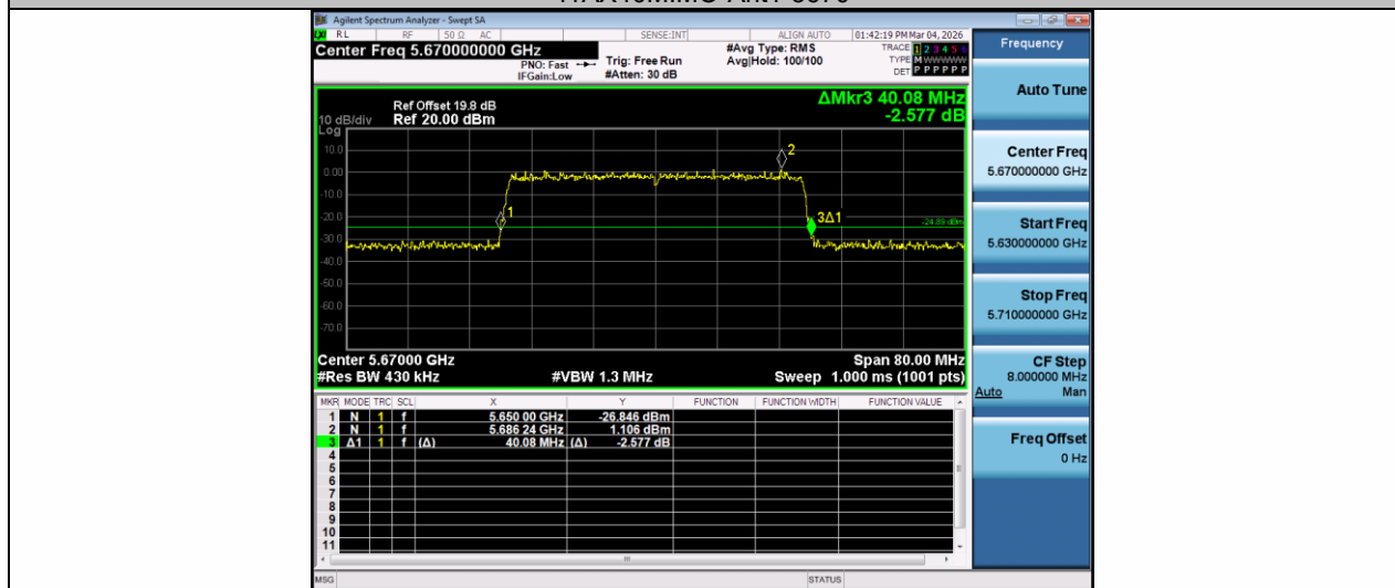
11AX40MIMO-Ant2-5670
