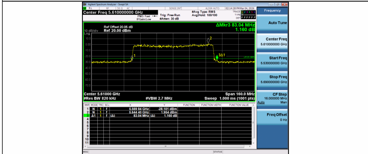
11AX80MIMO-Ant2-5610
