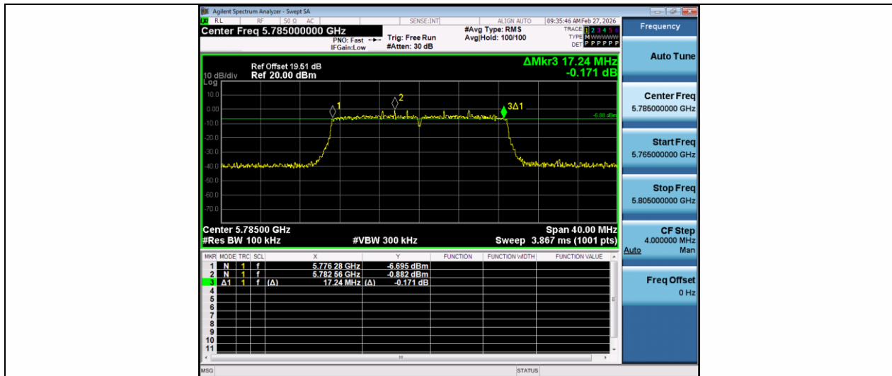
11N20MIMO-Ant2-5785-PASS
