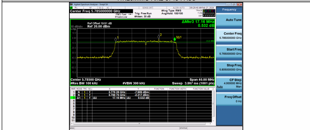
11N20MIMO-Ant1-5785-PASS
