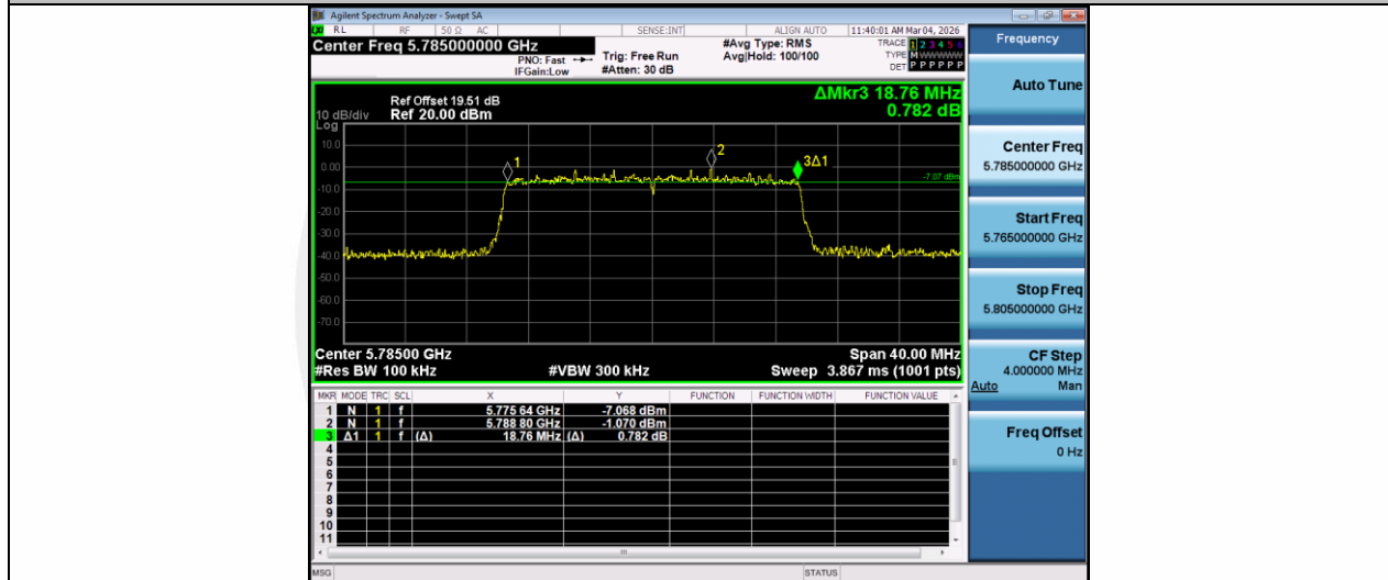
11AX20MIMO-Ant2-5785-PASS
