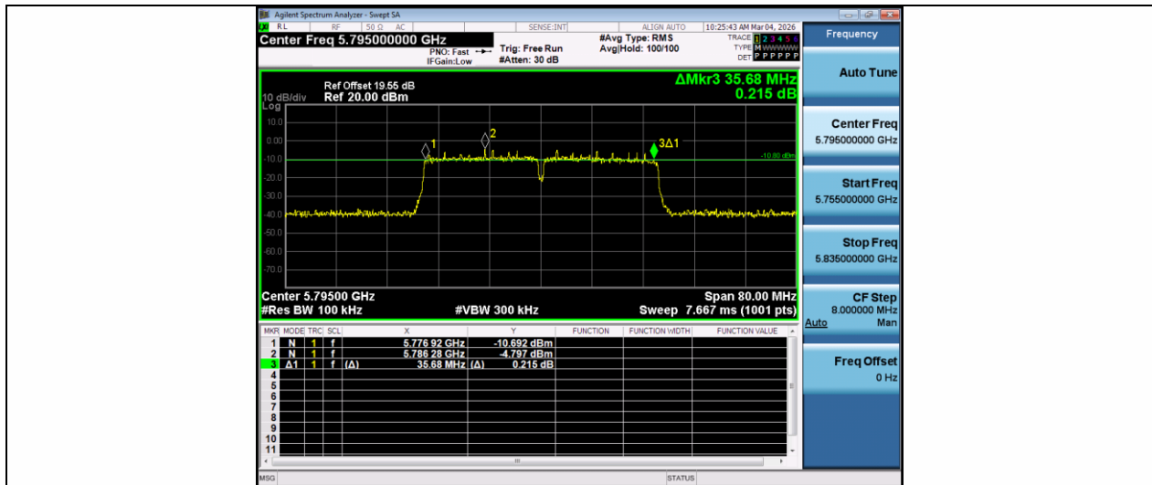
11AC40MIMO-Ant1-5795-PASS
