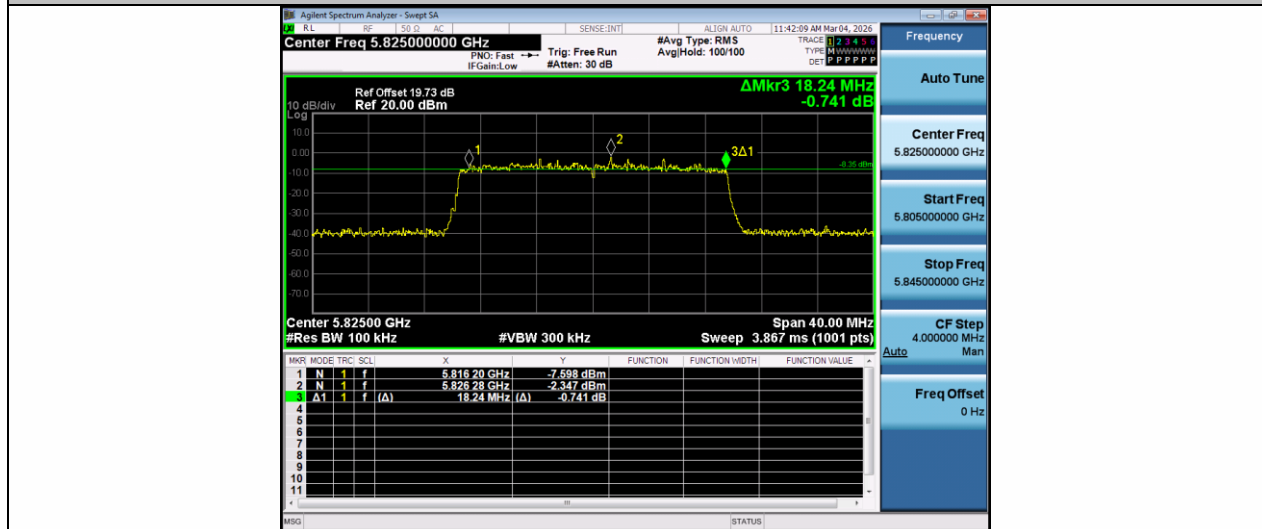
11AX20MIMO-Ant1-5825-PASS
