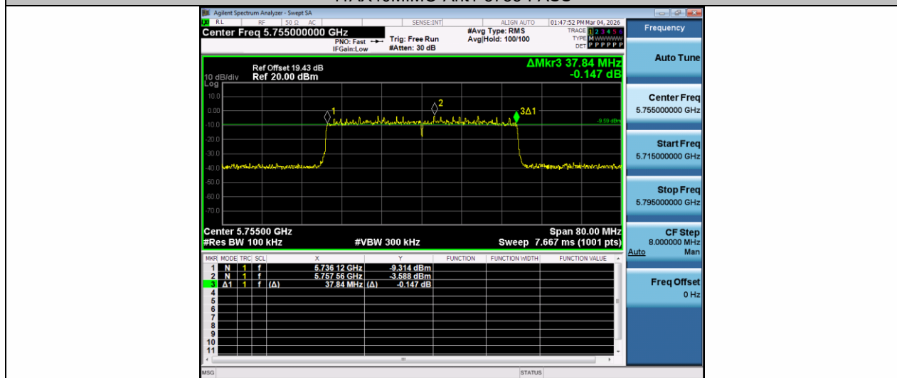
11AX40MIMO-Ant2-5755-PASS
