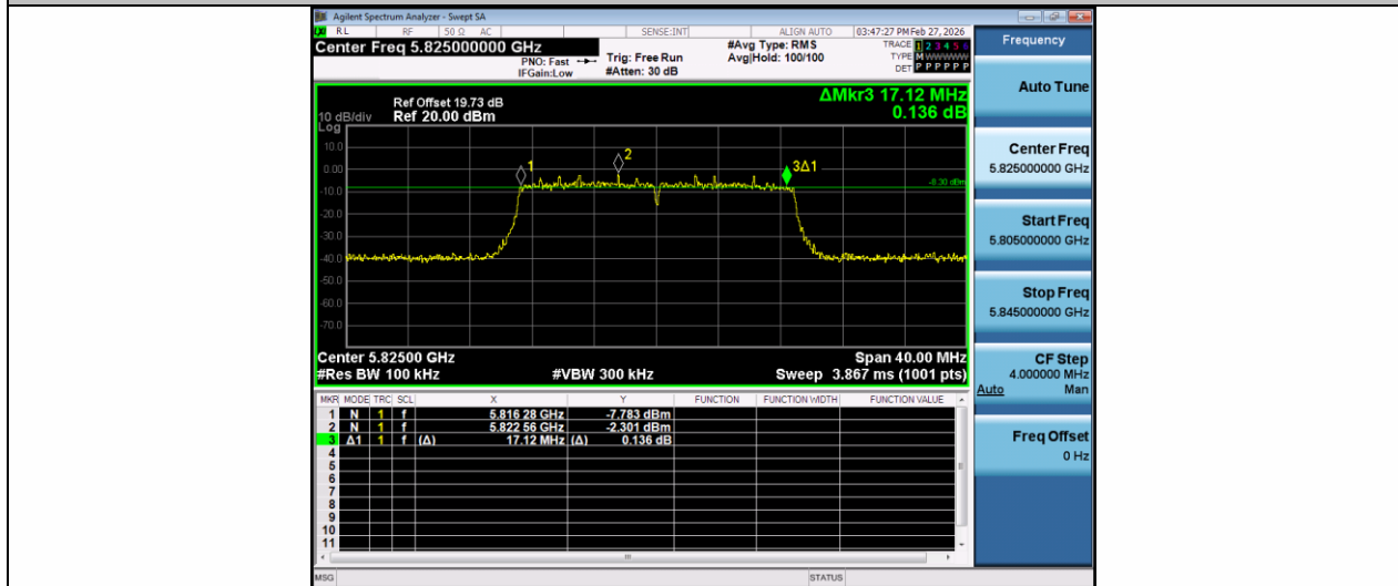
11AC20MIMO-Ant1-5825-PASS
