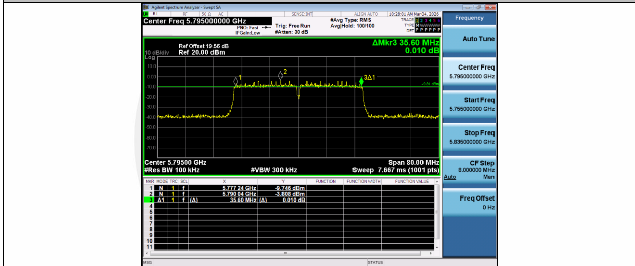
11AC40MIMO-Ant2-5795-PASS
