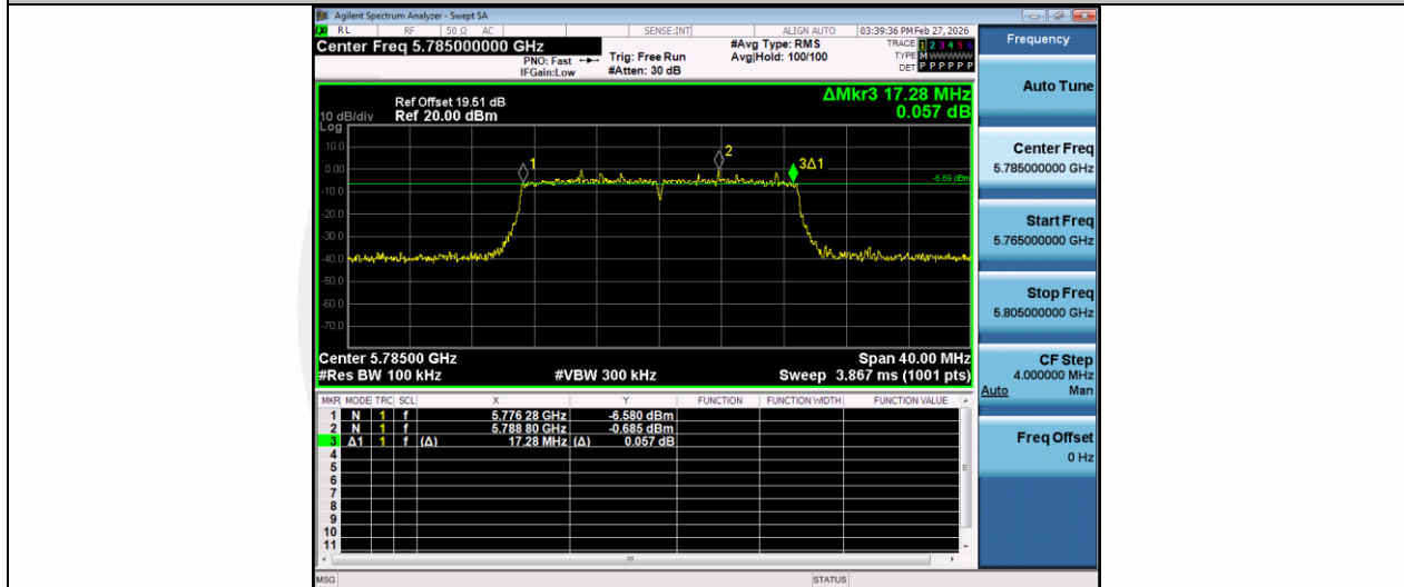
11AC20MIMO-Ant2-5785-PASS
