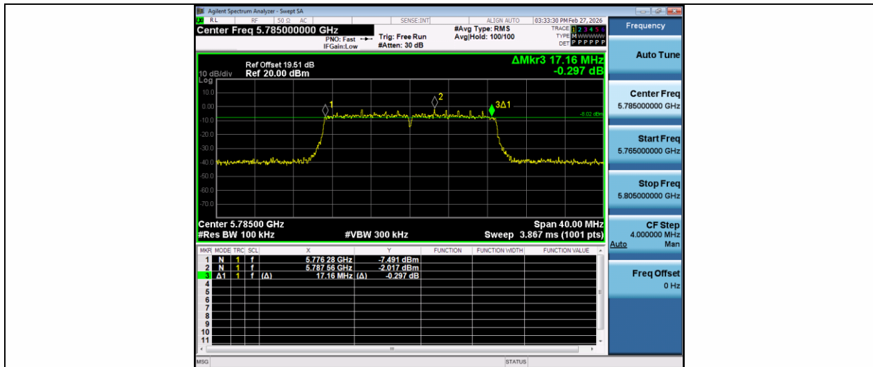
11AC20MIMO-Ant1-5785-PASS
