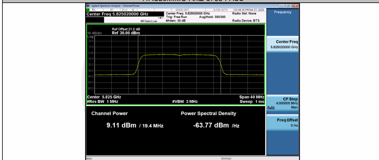
11AC20MIMO-Ant1-5825-PASS
