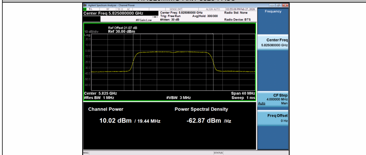
11AC20MIMO-Ant2-5825-PASS
