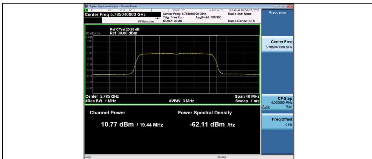
11AC20MIMO-Ant2-5785-PASS
