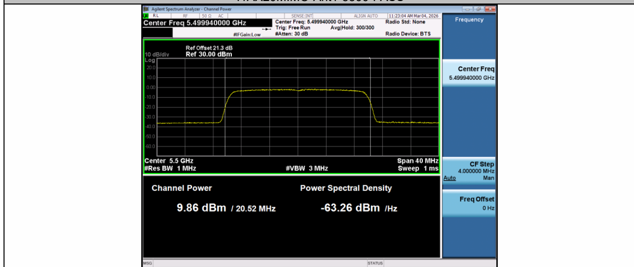
11AX20MIMO-Ant2-5500-PASS
