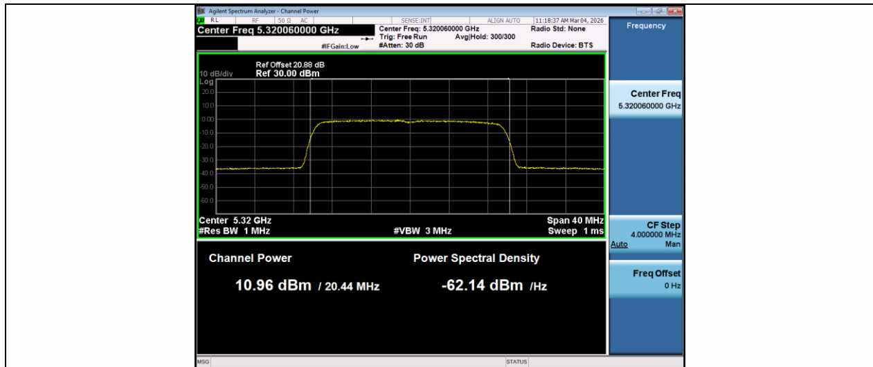
11AX20MIMO-Ant2-5320-PASS
