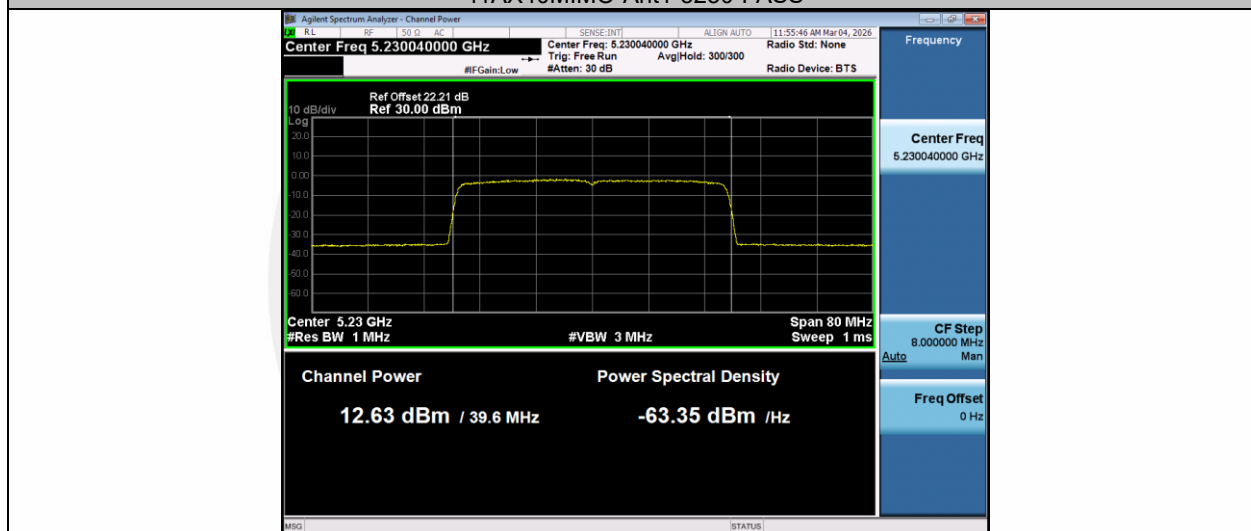
11AX40MIMO-Ant2-5230-PASS
