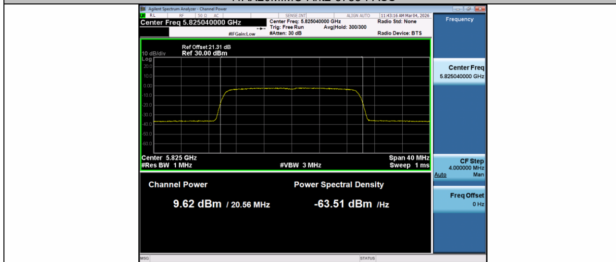
11AX20MIMO-Ant1-5825-PASS
