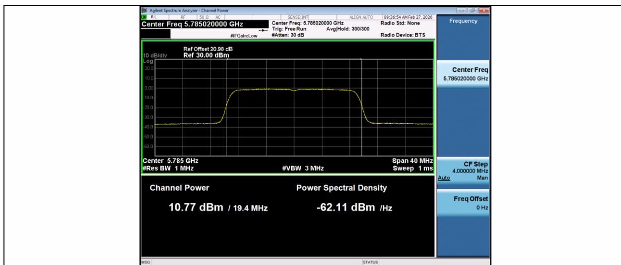
11N20MIMO-Ant2-5785-PASS
