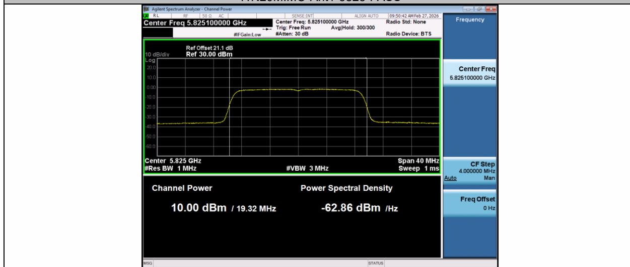
11N20MIMO-Ant2-5825-PASS
