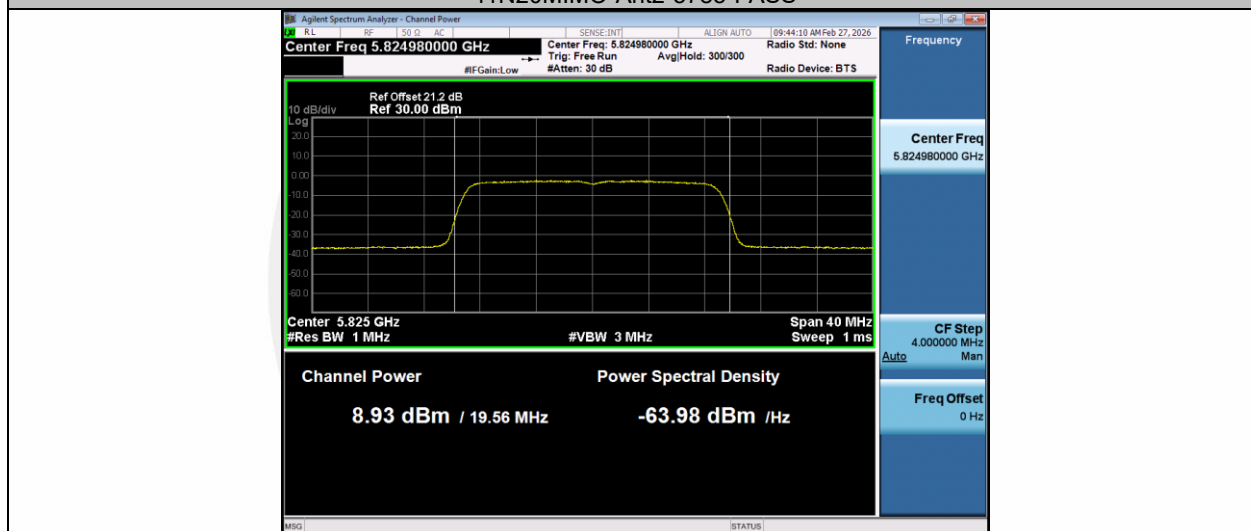
11N20MIMO-Ant1-5825-PASS
