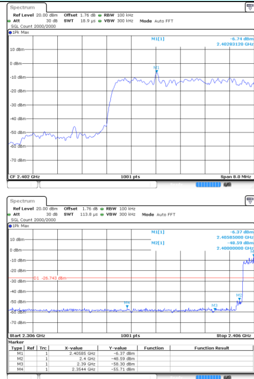
Hopping mode
