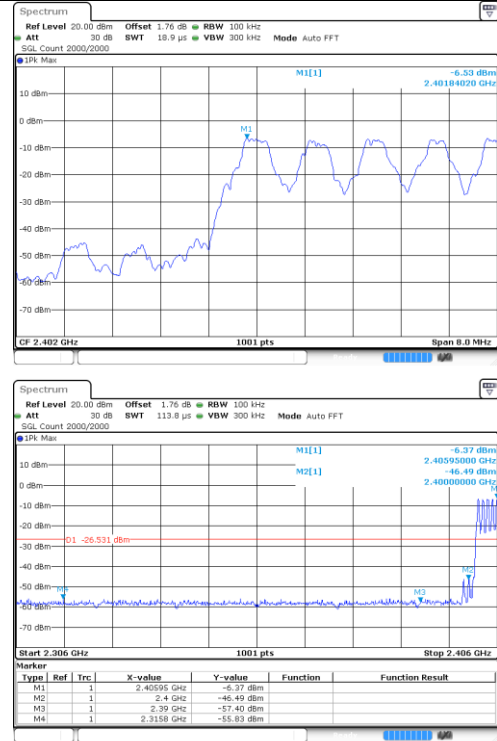
Hopping mode
