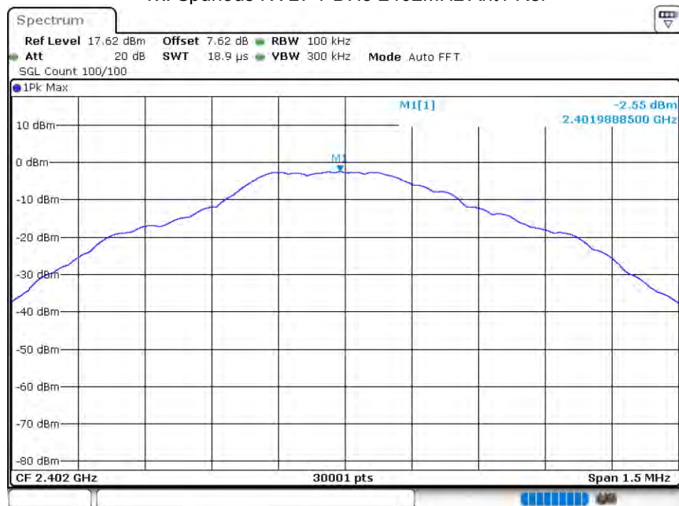
Tx. Spurious NVLT 1-DH5 2402MHz Ant1 Ref
