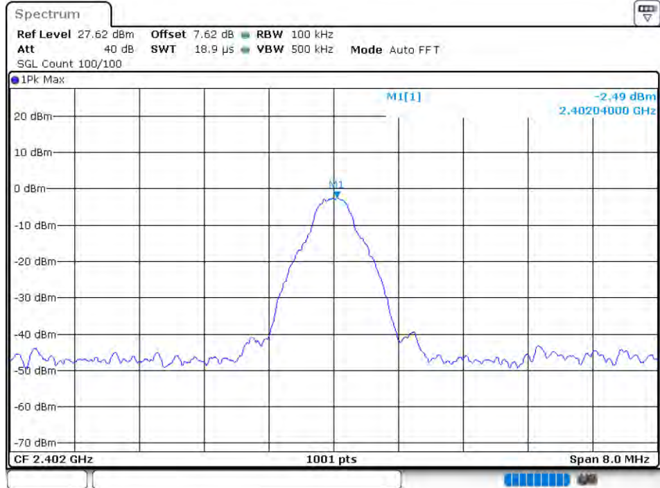
Band Edge NVLT 1-DH5 2402MHz Ant1 No-Hopping Ref
