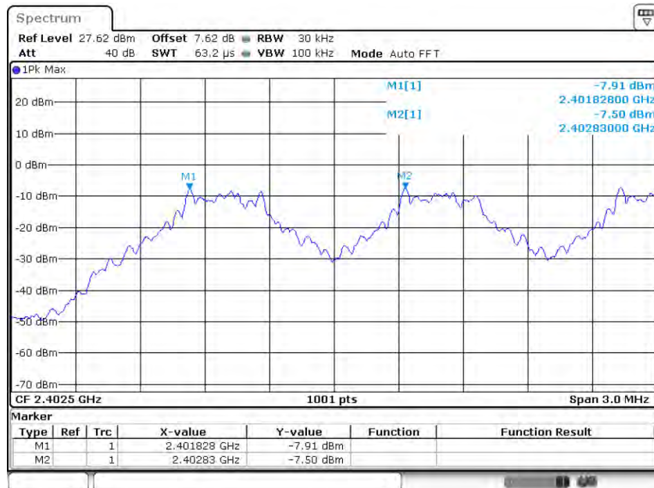
CFS NVLT 1-DH5 2402MHz
