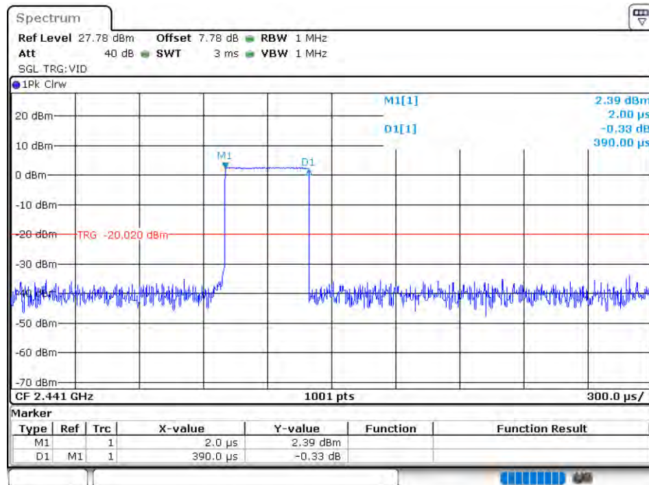
Dwell NVLT 1-DH1 2441MHz
