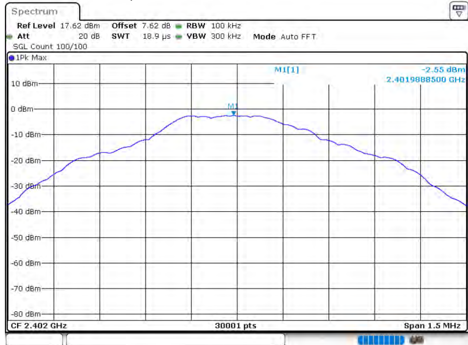
Tx. Spurious NVLT 1-DH5 2402MHz Ant1 Ref
