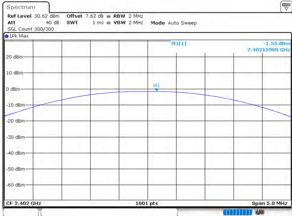
Power NVLT 1-DH5 2402MHz Ant1
