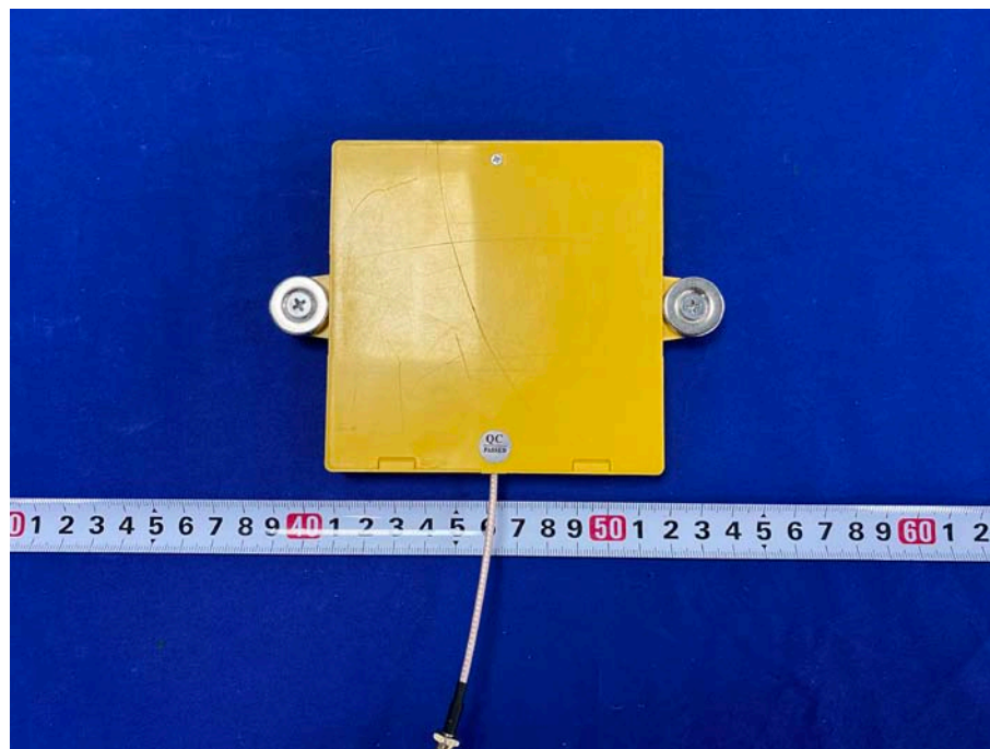
Antenna Bottom View
