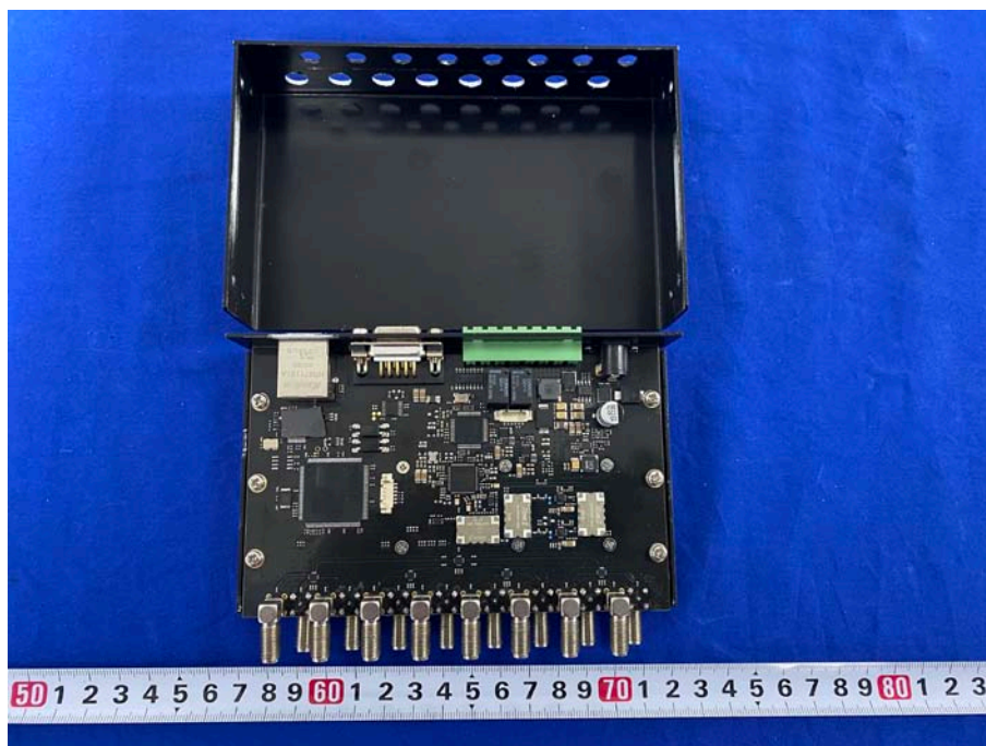
Uncovered View
